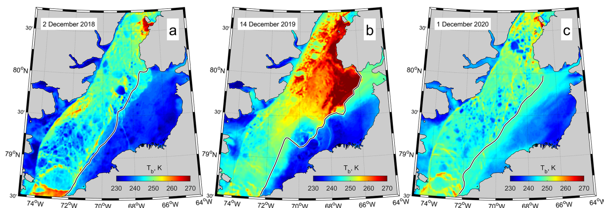
Figure 10. MODIS clear-sky brightness temperatures on (a) 2 December 2018, (b) 14 December 2019 and (c) 1 December 2020. Images (b) and (c) show T_b several days prior to ice bridge formations in both years. The black lines indicate approximate positions of the landfast ice edge at the date of each imagery.
