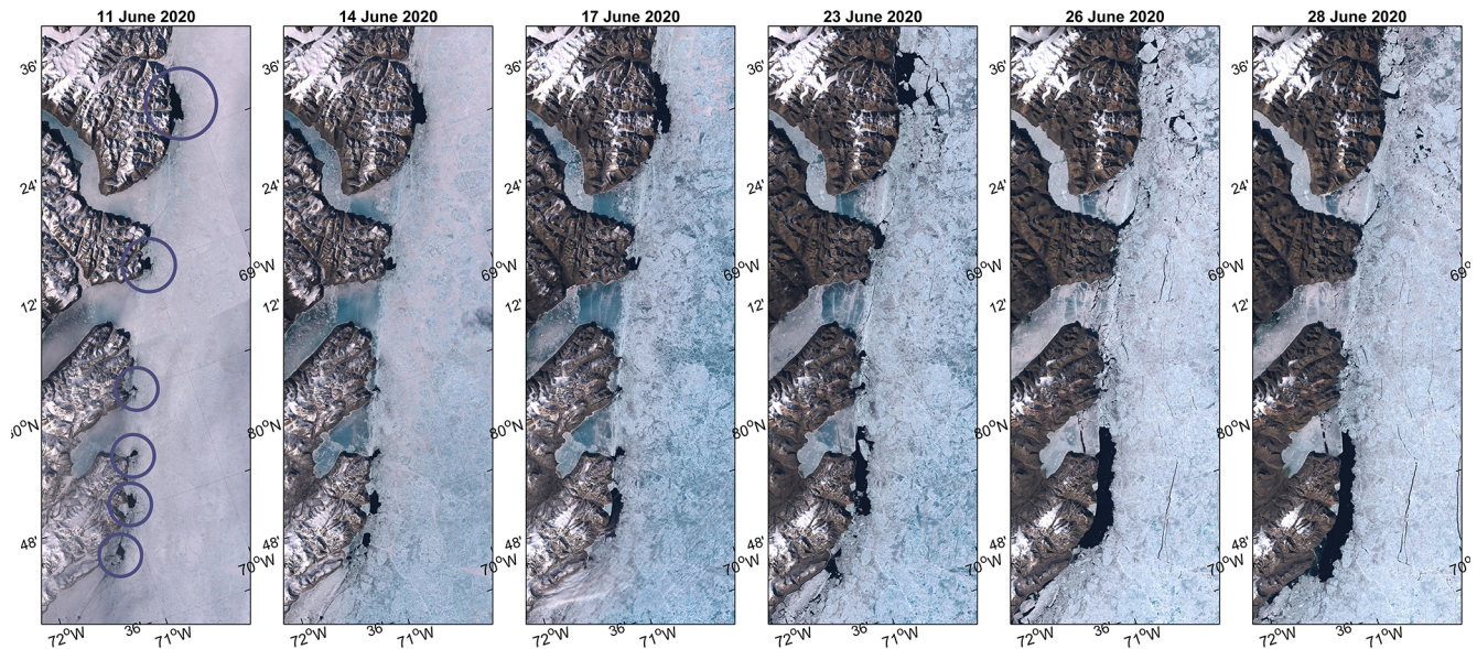
Figure 11. The series of Sentinel-2 images showing the evolution of polynyas along the western coast of Kane Basin from their first appearance until the start of bridge collapse in June 2020. The circles in the leftmost panel indicate the regions where open-water polynyas first appear.
