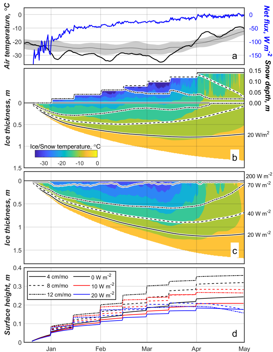
Figure 6. (a) The 2 m air temperature (black) and the net surface heat flux (blue). Gray line and shading indicate the mean 1979–2020 temperature and standard deviation. (b) The modeled evolution of ice and snow temperature and thickness in the vicinity of polynya under a constant snowfall rate of 4 cm per month (corresponding to 14 cm of snowpack at the end of March). (c) The same as (b) but under no-snow conditions – a proxy of the polynya at Cape Jackson. Black lines in (b) and (c) show the evolution of ice and snow thicknesses if an additional heat flux of 20 (solid), 40 (dashed), 70 W m^{-2} (dashed–dotted) or 200 W m^{-2} (dotted) from below is applied. (d) The calculated difference between the sea surface in ice-free polynya and the combined surface heights of ice and snow within surrounding ice for different snow accumulation rates and ocean heat fluxes.
