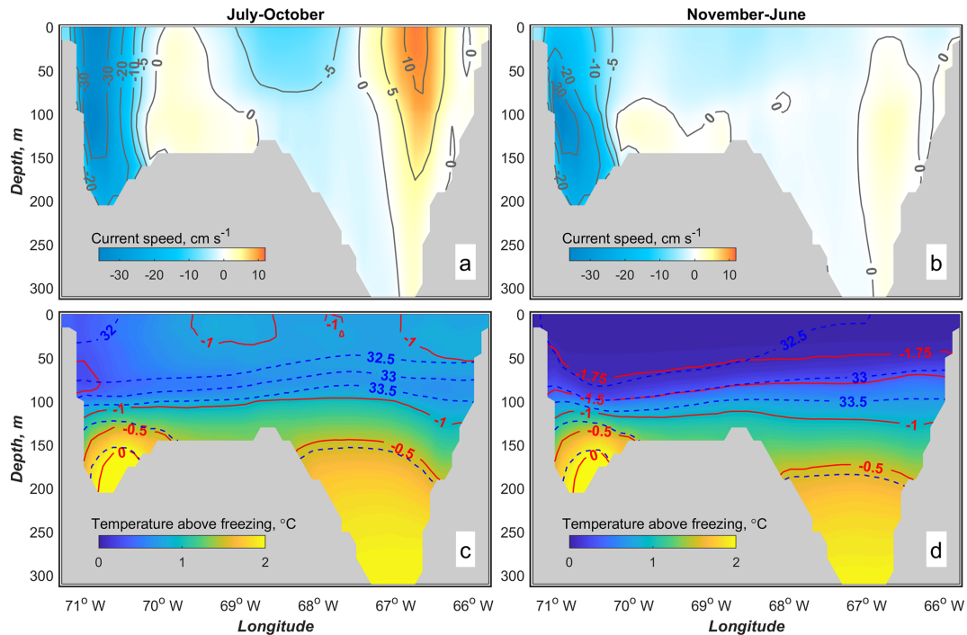
Figure 9. The modeled mean 2006–2010 summer (mobile ice) and winter (ice bridge) cross-sectional current speed ( a , b ) and water temperatures and salinities ( c , d ) at the transect across the central Kane Basin. Positive speeds correspond to northward flow.
