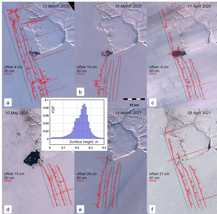
Figure 3. The ATL07 elevations (red lines) from three strong beams overlaid on Sentinel-2 images of the polynya in March–May 2020 and in March–April 2021. The elevations are adjusted to the sea level in the polynya and plotted as absolute deviations from the ground tracks (black lines) in a direction normal to the tracks. The open water was used as a reference level to calculate the corresponding offsets for each subset. The red scale bar in each panel corresponds to 50 cm elevation. The inset histogram demonstrates the probability distribution of all heights shown in (a)–(f).
