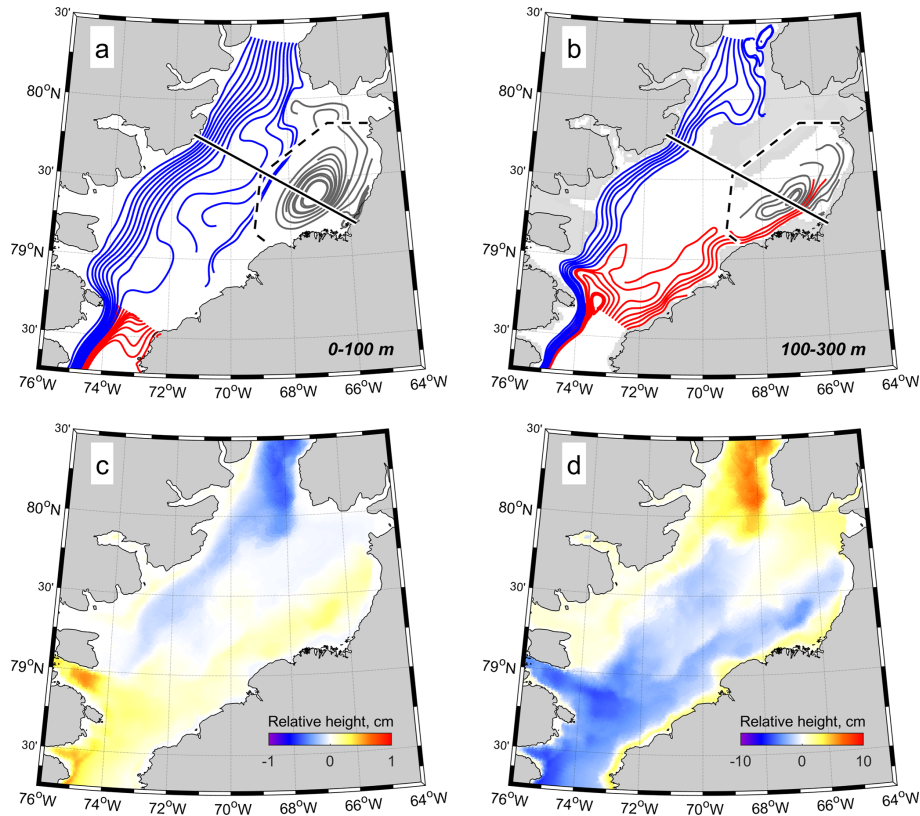
Figure 7. (a–b) The trajectories of water parcels calculated from the mean 2006–2010 model current velocities averaged within 0–100 and 100–300 m, respectively. The blue, red and gray lines correspond to three main circulation patterns in the region (see more details Sect. 3.4). The black dashed line envelopes the region used for vorticity calculation (Fig. 8) and the solid line shows the position of transect presented in Fig. 9. The shaded area in (b) corresponds to the regions shallower than 150 m. The spatial distribution of the mean winter (November–June) thermosteric and halosteric sea level anomalies is shown in (c) and (d), respectively.
