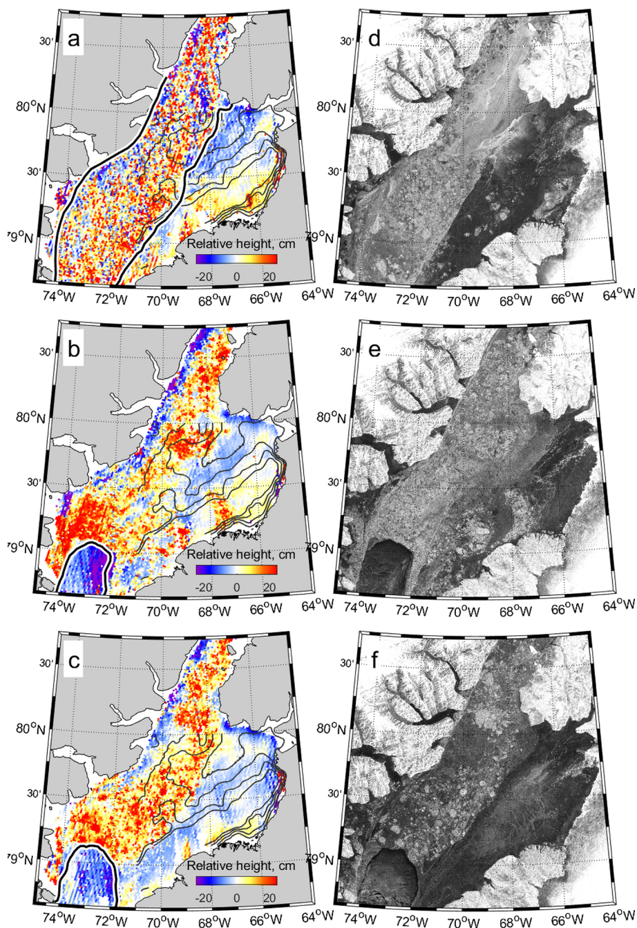
Figure 4. (a–c) The along-track anomalies of ATL07 elevations averaged over 1.5 \times 1.5 km cells in January–April 2019 (a), 2020 (b) and 2021 (c). The thick black lines correspond to approximate positions of landfast ice edge during these winters. (d–e) Sentinel-1 SAR images from 16 January in the corresponding years.
