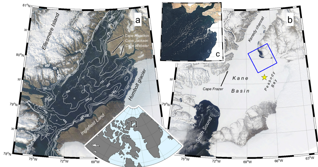
Figure 1. (a) The bathymetry of the central part of Nares Strait with contours corresponding to 100, 150, 200, 250 and 300 m isobaths overlaying on the true-color MODIS imagery from NASA Worldview. (b) The MODIS image of the sensible polynya at Cape Jackson on 6 June 2021. The blue square borders a region shown in Fig. 2, and the yellow star shows the position of ERA-5 reanalysis data used in the ice growth model. (c) The high-resolution Sentinel-2 image showing the chains of grounded icebergs in the northern Peabody Bay on 8 September 2019.
