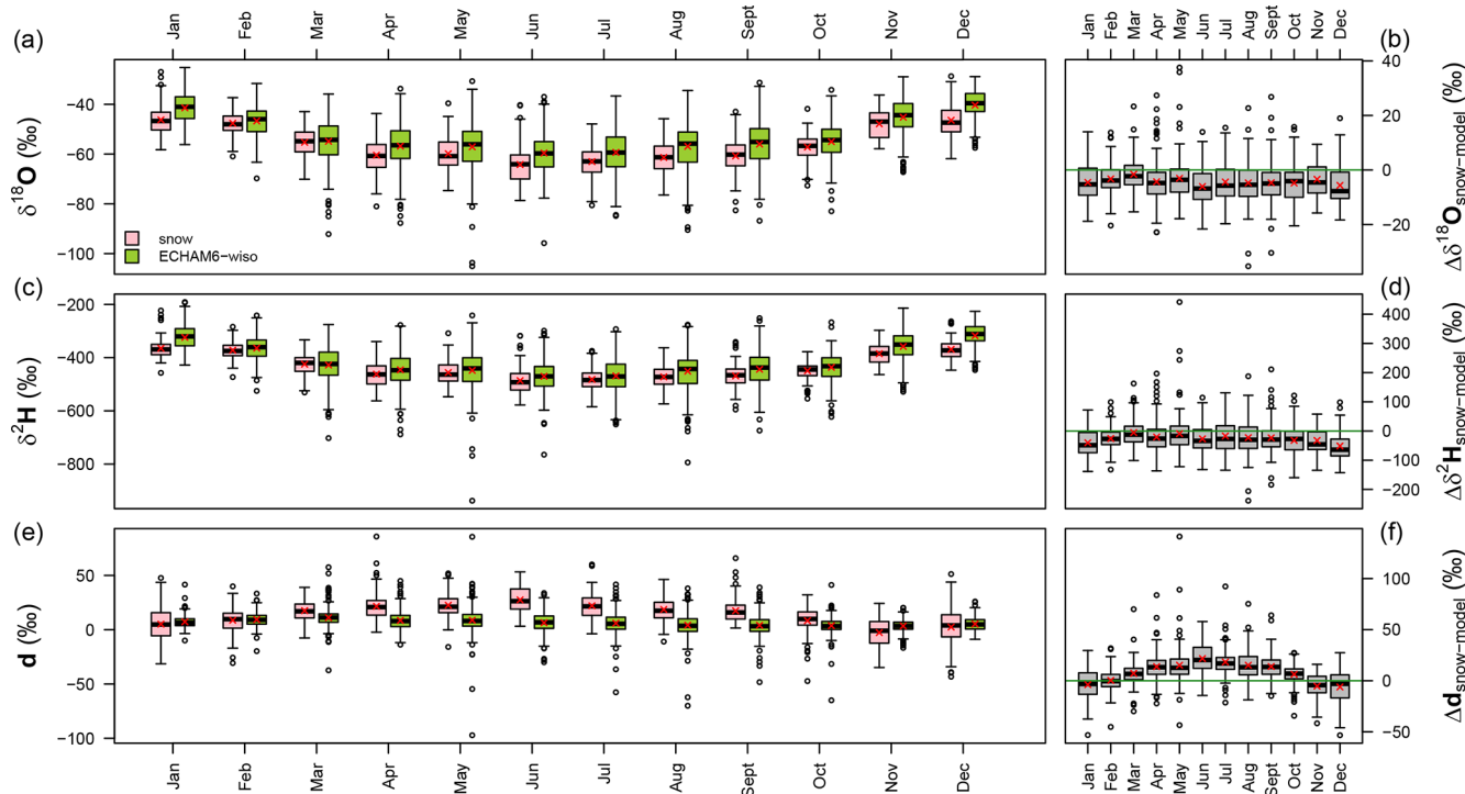
Figure 7. Seasonal variation of the experimentally measured isotopic data and ECHAM6-wiso modeled data (a, c, e) and their differences (b, d, f). Line: median, box: interquartile range, whiskers: \pm 1.5 interquartile range, circles: outliers and extremes, red crosses: arithmetic mean.
