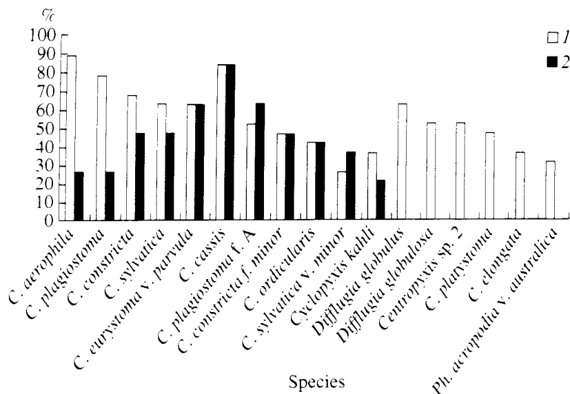
Fig. 2. Dominant complex of testaceans (occurrence > 30%) in Holocene and Late Pleistocene sediments of Bykovsky Peninsula; 1, Holocene; 2, Pleistocene.
