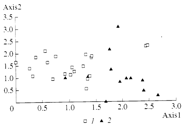
Fig. 5. Results of undirected correspondence analysis of Late Pleistocene and Holocene samples of Bykovsky Peninsula; 1. Pleistocene; 2. Holocene.
