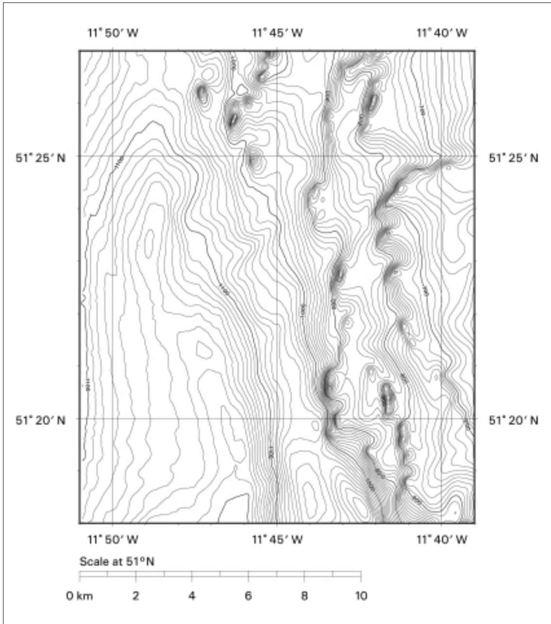
Figure 4: Section from the mound area of the Porcupine Seabight
