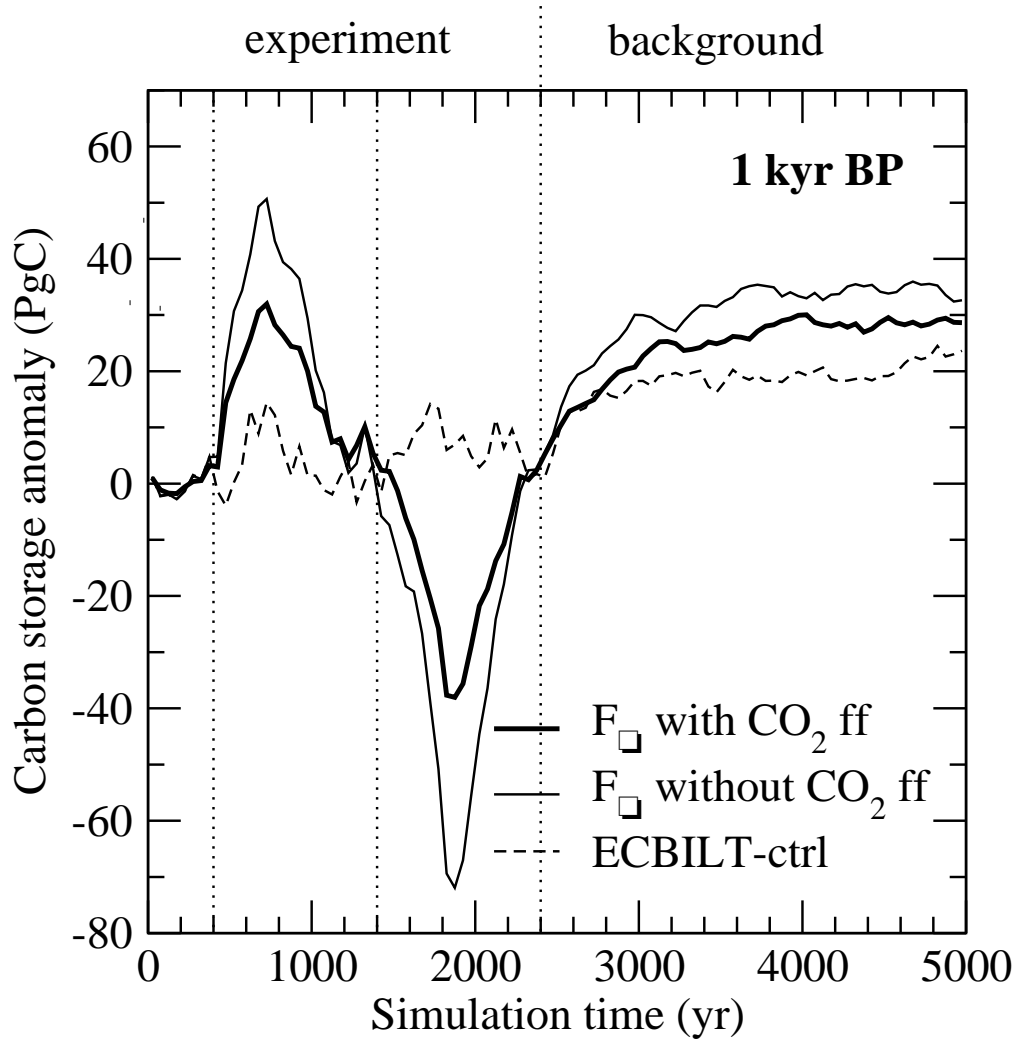
Fig. 8. Change in global terrestrial carbon storage versus time simulated by the LPJ-DGVM in response to the climate perturbations of the ECBILT-CLIO freshwater experiment F_{\square} (Fig. 2) and preindustrial (1 kyr BP) initial conditions. Results are shown for experiments with (solid) and without (thin) \text{CO}_2 fertilisation feedbacks (ff) and for a control (dash) without freshwater discharge and without \text{CO}_2 fertilisation feedbacks. Vertical lines at 400 yr and 1400 yr indicate the beginning and the end of the freshwater discharge in ECBILT-CLIO. After year 2400 the LPJ-DGVM was again forced with the initial climate conditions.
