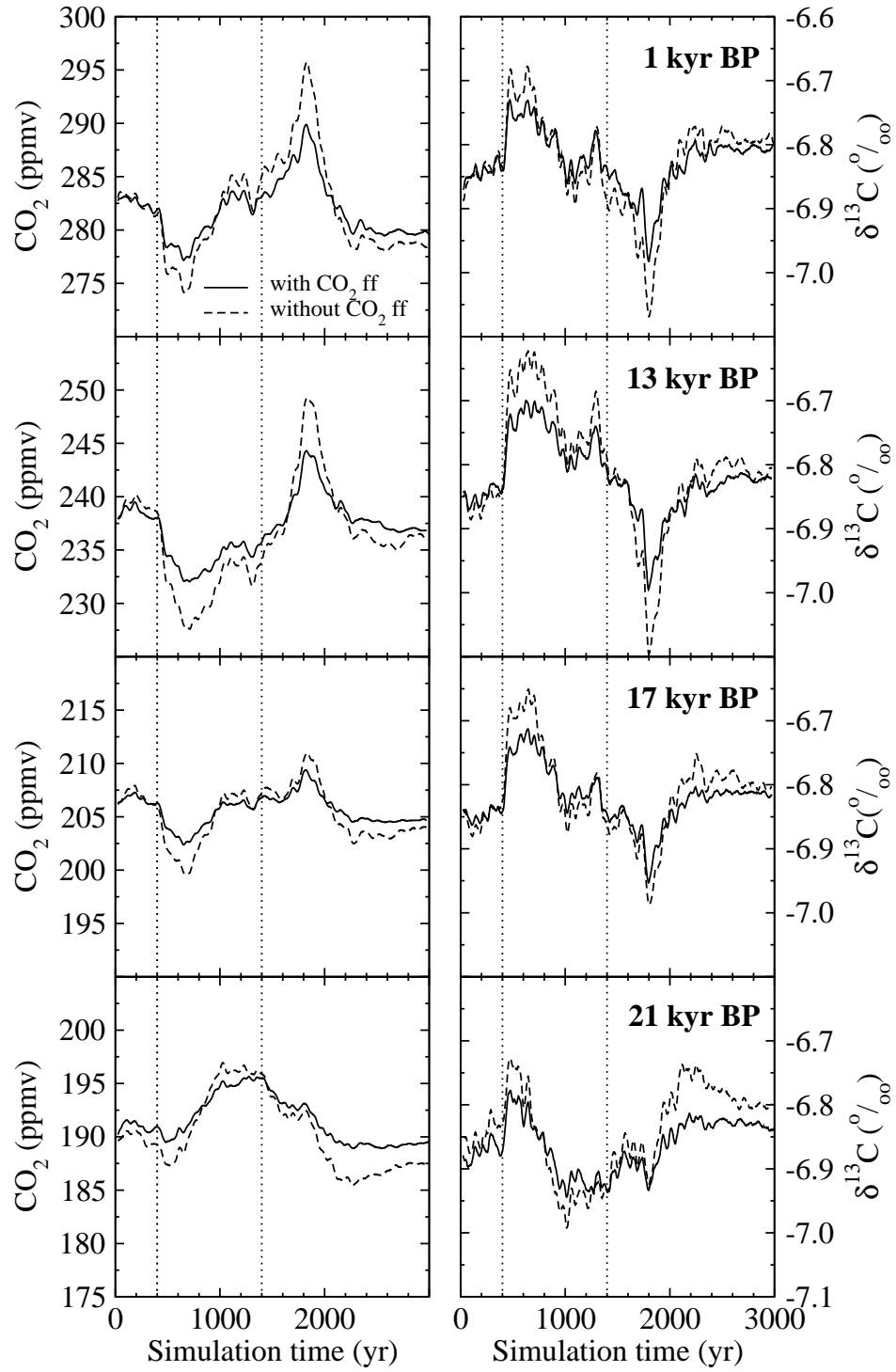
Fig. 9. Anomalies in atmospheric \text{CO}_2 (left) and \delta^{13}\text{C} (right) for different initial conditions ( t = 1, 13, 17 , and 21 kyr BP) as simulated with the LPJ-DGVM in response to the scenario F_{\square} and for simulations with (solid) and without (dash) \text{CO}_2 fertilisation feedbacks (ff). Vertical lines at 400 yr and 1400 yr indicate the beginning and the end of the freshwater discharge.
