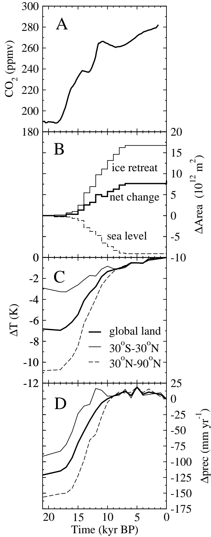
Fig. 3. Changes in climate boundary conditions over the past 21 kyr. A: \text{CO}_2 from EPICA Dome C (Monnin et al., 2001) synchronised via \text{CH}_4 to the GISP2 age scale and splined (Köhler et al., 2005). B: Changes in land available for plant growth relative to 21 kyr BP in response to ice sheet retreat and sea level rise and the resulting net change (Peltier, 1994). C, D: Temperature and precipitation anomalies over land area (excluding Antarctica) as simulated with the Hadley Centre HadSM3 climate model for time slice experiments about every 1 kyr and linear interpolation between them, globally averaged and for different latitudinal bands (sub-figures B, C, D adapted from Joos et al., 2004)
