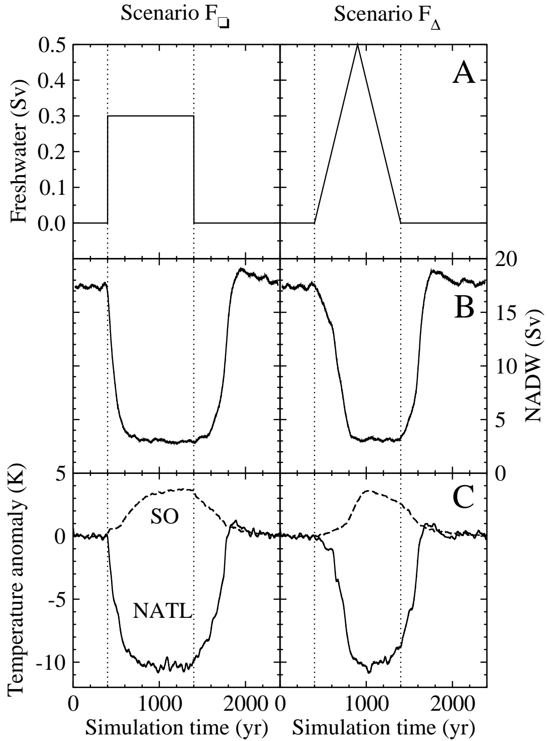
Fig. 2. Freshwater discharge into the North Atlantic ( 50^{\circ}\text{N} – 70^{\circ}\text{N} ) prescribed in simulations with the ECBILT-CLIO climate model (A), and the simulated change in North Atlantic Deep Water (NADW) exported at 30^{\circ}\text{S} (B) and in near surface air temperature of the whole North Atlantic region (NATL, 60^{\circ}\text{W} – 20^{\circ}\text{E} , 50^{\circ}\text{N} – 80^{\circ}\text{N} ), and the Southern Ocean (SO, 65^{\circ}\text{S} – 50^{\circ}\text{S} ) (C) for scenario F_{\square} (left) and F_{\Delta} (right).
