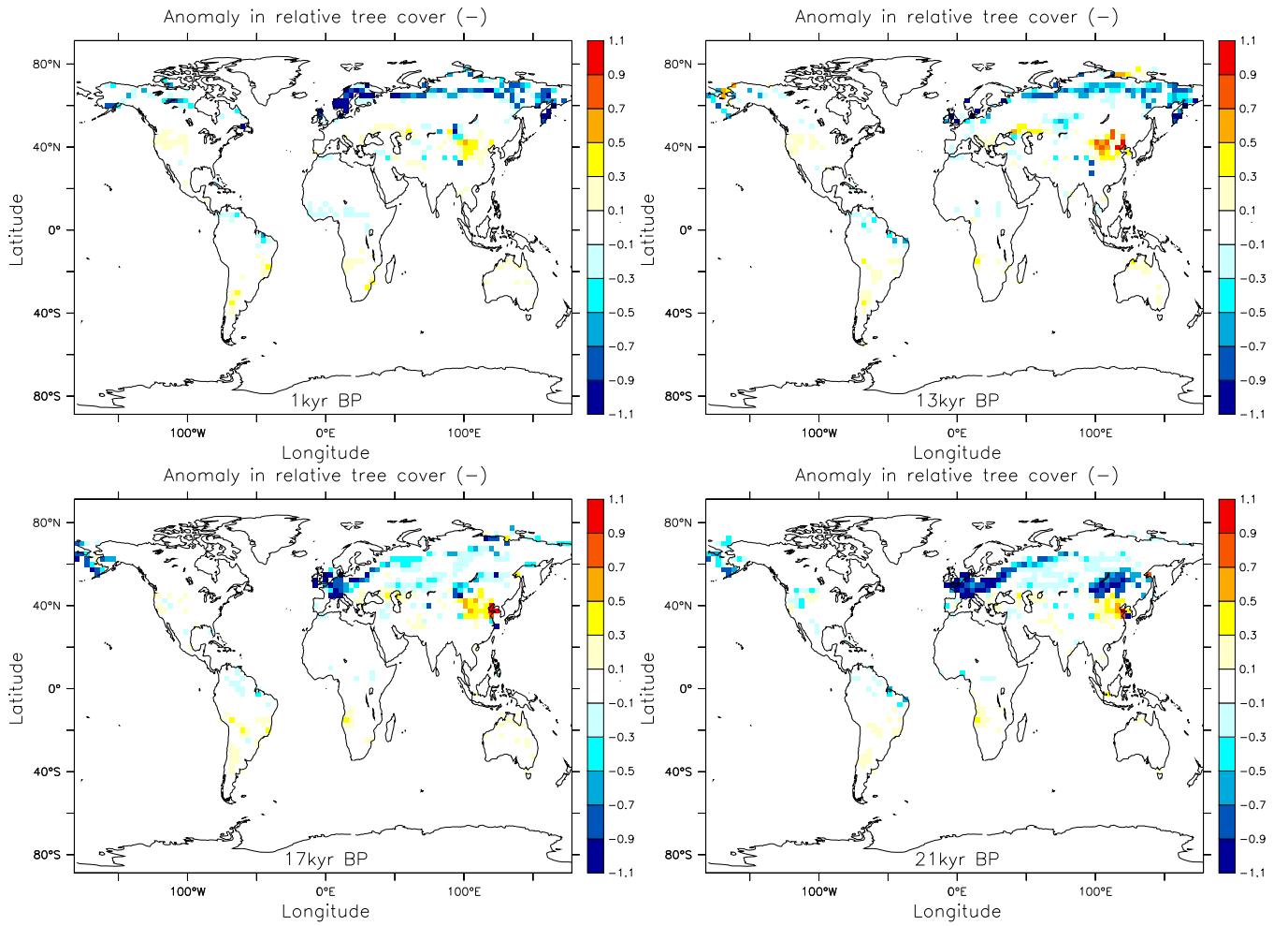
Fig. 7. Anomalies in the relative tree cover for scenario F_{\square} and different initial conditions ( t = 1, 13, 17 , and 21 kyr BP). The anomaly is calculated as average distribution during the peak cold phase ( t = 1001 - 1400 yr) with respect to the first 400 yr of the simulation, i.e. before the start of the freshwater discharge in ECBILT-CLIO. These model results are largely independent of \text{CO}_2 fertilisation feedbacks. Results shown are from simulations without \text{CO}_2 fertilisation feedbacks. Blue colours indicate a loss of relative tree coverage and yellow-red colours a gain relative to the average of the first 400 yr.
