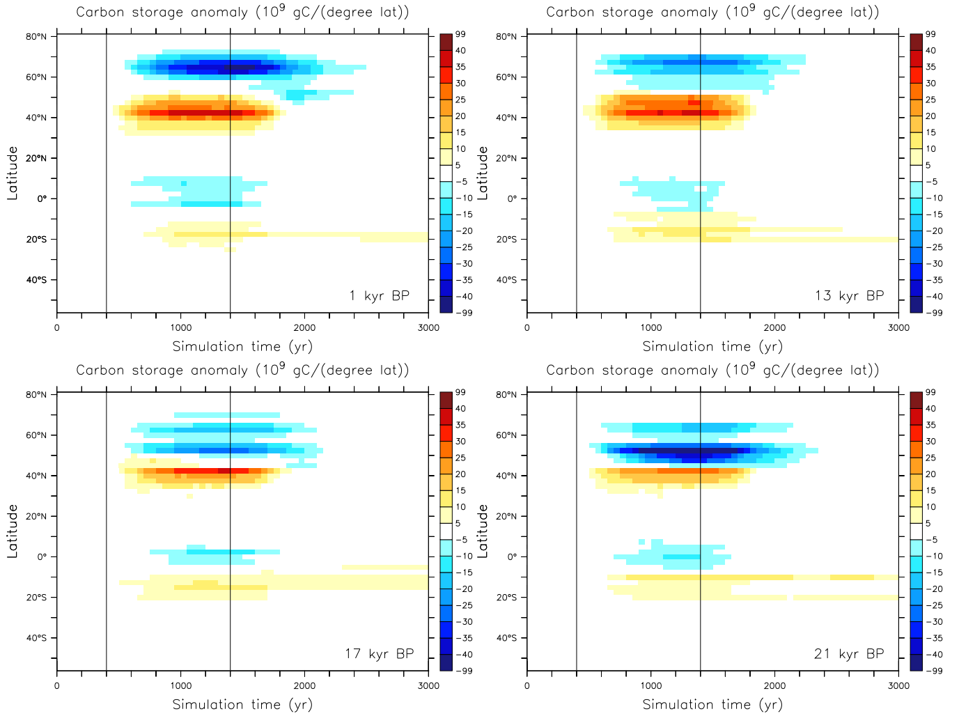
Fig. 12. Zonally-averaged anomalies in total land carbon storage versus time for different initial conditions ( t = 1, 13, 17 , and 21 kyr BP) as simulated by the LPJ-DGVM under constant \text{CO}_2 (no \text{CO}_2 fertilisation feedbacks) and using ECBILT-CLIO climate anomalies from experiment F_{\square} . Vertical lines at 400 yr and 1400 yr indicate the beginning and the end of the freshwater discharge in ECBILT-CLIO. Blue colours indicate a loss of carbon and yellow-red colours a gain of carbon relative to the average of the first 400 yr.
