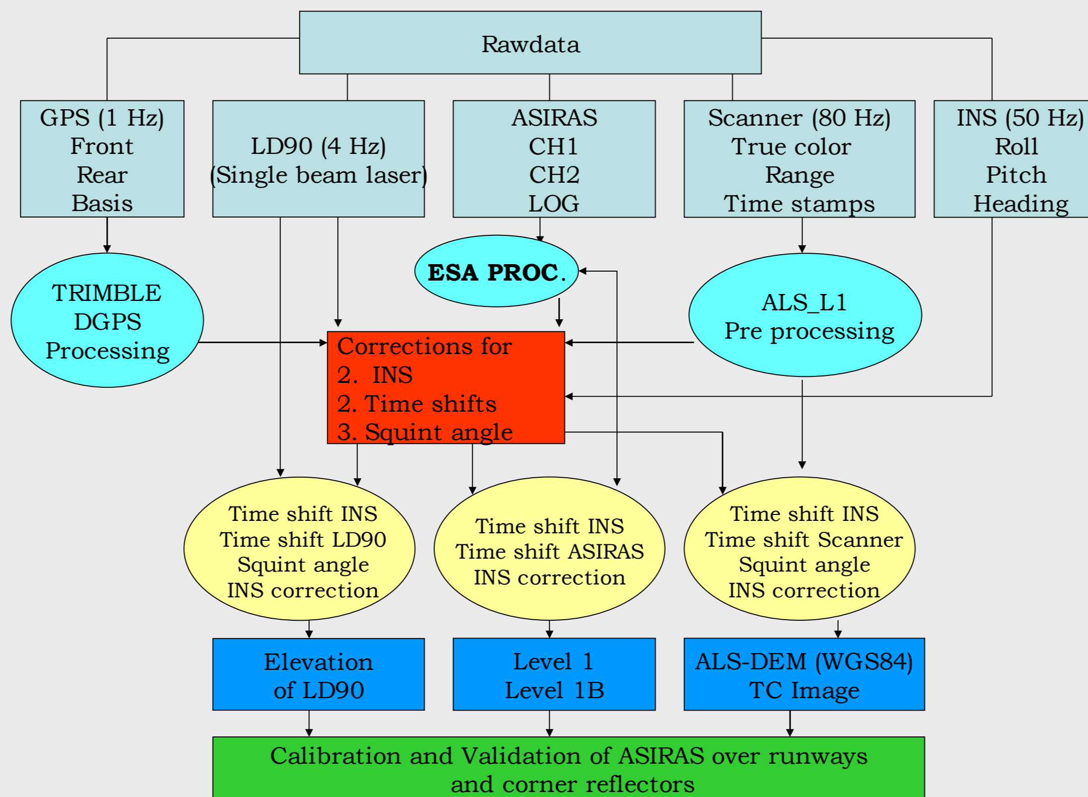
Figure 4: Cal/Val processing flow of ASIRAS
