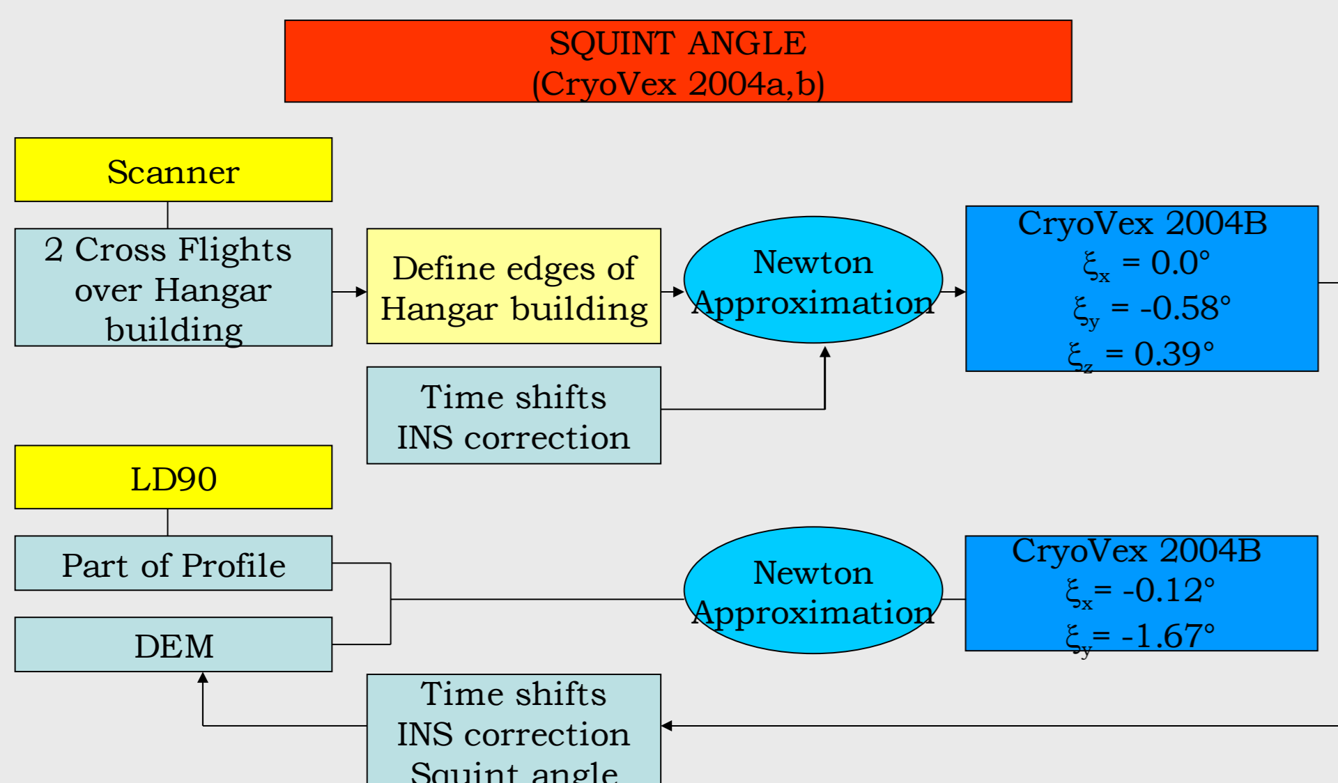
Figure 6: Concept of the determination of squint angles
