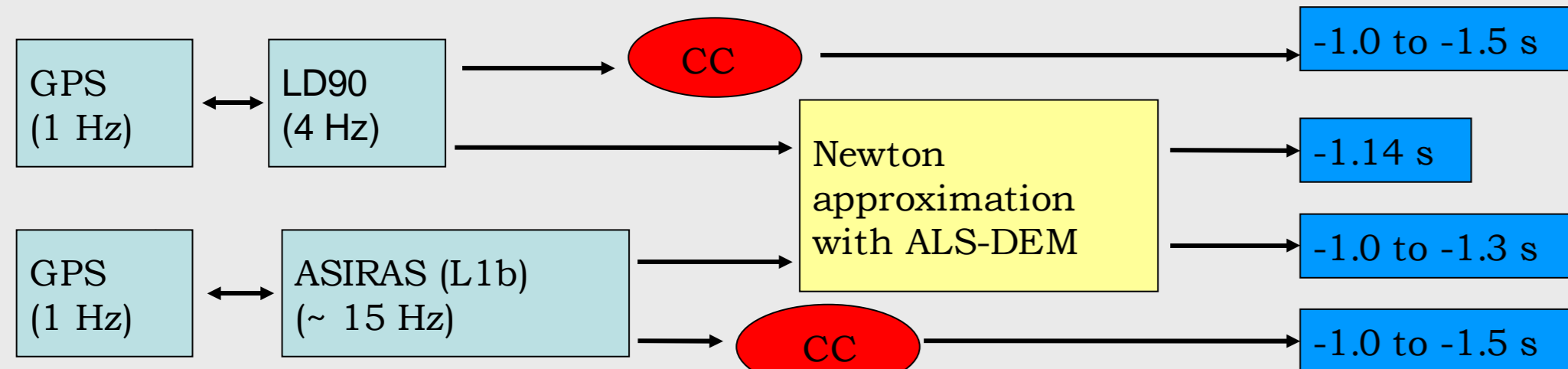
Figure 5: Concept of the determination of time shifts
