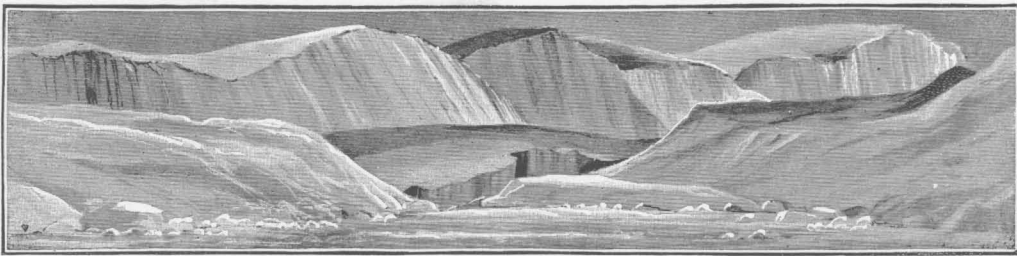
FIG. 8. GLACIER ENTERING VALLEY. THE CLIFFS TO THE RIGHT ARE AT THE HEAD OF THE FIORD (ANTOINETTE BAY). MAY 12, 1883.
