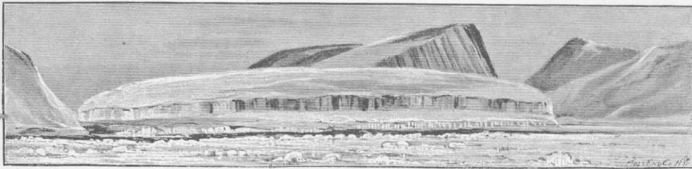
FIG. 1. FACE OF GLACIER ABOVE EMMA BAY (FROM TENT). APRIL 30, 1883.
