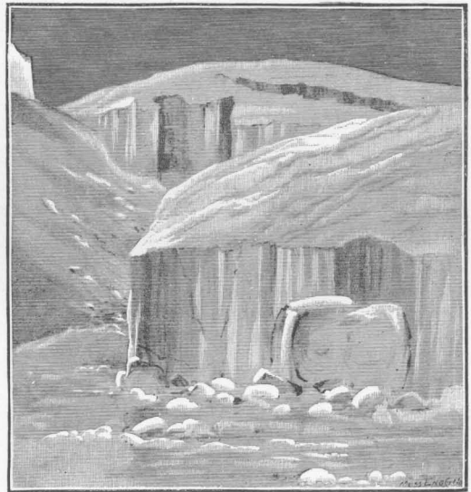
FIG. 6. OFF-SHOOT OF THE MER DE GLACE. THE SAME AS FIG. 8. THE HILL-SIDES ON THE LEFT CORRESPOND. NEAR HEAD OF LAKE BETWEEN CAMPS XII AND XIII. MAY 12, 1883.
