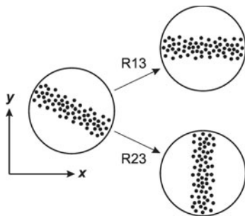
Fig. 8. Sketch of the rotation of the girdle fabrics in order to align them with the x axis (case R13) and the y axis (case R23) in the Schmidt projection.
