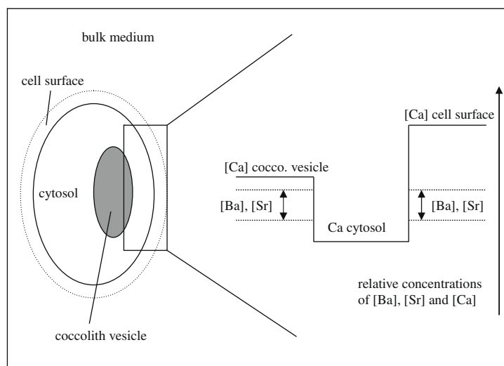
Fig. 4. Proposed mechanism for the partitioning of Sr, Ba and Ca during calcification in Emiliana huxleyi yielding the K_{D_{Sr}}^B , and K_{D_{Ba}}^B . Depicted are the relative concentrations of Sr, Ba, and Ca in the two involved cellular compartments (coccolith vesicle and cytosol) and the cell surface. The Sr and Ba concentrations (dashed lines) at the cell surface and in the coccolith vesicle increase until the thermodynamical limit of the concentration gradient between the cytosol and adjacent compartments is reached. The same holds for the Ca concentration (solid lines) at the cell surface. However, the Ca concentration in the coccolith vesicle is determined by the saturation product. All variations of the Sr and Ba concentrations at the cell surface are reflected by variations of the Sr and Ba concentrations in the coccolith vesicle (as indicated by the double-headed arrows).
