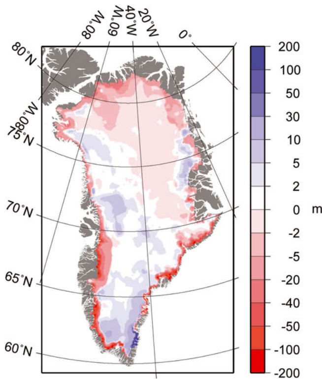
Fig. 4. Spatial pattern of total cumulated surface mass-balance change for the period 1866–2005. Values are in metres ice equivalent.
