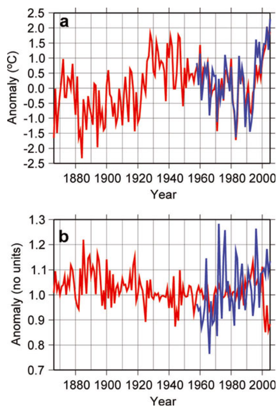
Fig. 2. (a) Mean annual temperature (TMA) difference averaged over ice-sheet area, assembled from two datasets: ECMWF re-analyses (blue) and BOX (red). (b) Annual precipitation ratio averaged over ice-sheet area. Colour convention as in (a).
