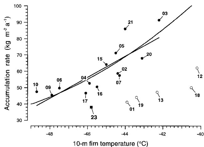
Fig. 7. Relationship between accumulation rate and 10 m firn temperature. The straight line gives the regression line through the data points. The curve represents the fit of a function, which is proportional to the temperature derivative of the mixing ratio, to the data points. The accumulation rates are proportional to the water-vapour loss from a cooling air mass. The data from sites marked by open symbols were omitted in the fitting procedures.
