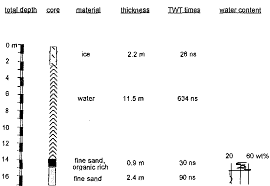
Figure 3-4: Coring results for the lake sediment site, the respective material thicknesses and the deduced TWT times in the GPR section.
