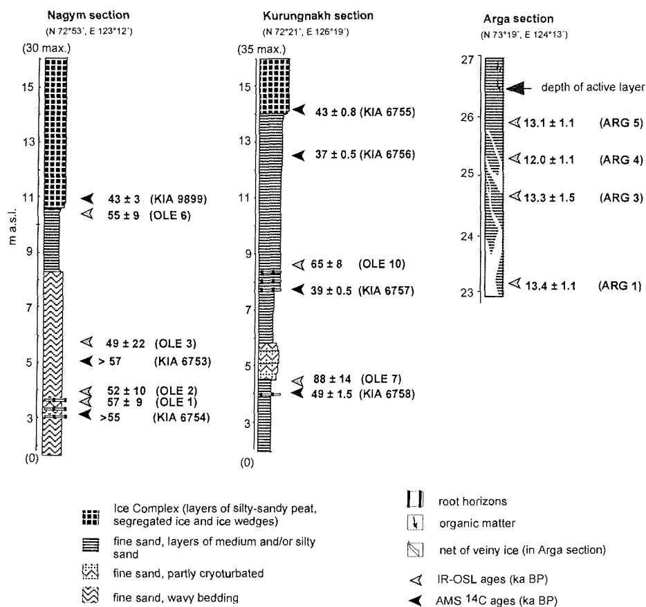
Figure L-4: Scheme of the sediment sequences investigated, compiled with the IR-OSL and ^{14}\text{C} age data.
