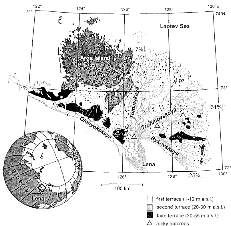
Figure 1-1: Geomorphologic overview of the Lena Delta according to Grigoriev (1993). Values for the river runoff in the major delta branches are added after Alabyan et al. (1995).
