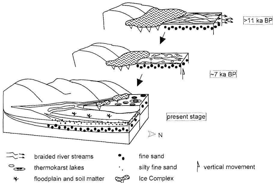
Figure 5-2: Tectono-sedimentary evolution of the Lena Delta during Late Pleistocene and Holocene with emphasis on the western sector. Ice Complex deposition along the foots of the highlands was followed by lateral and vertical sedimentation of a braided Lena river run-off shortly before the termination of the Pleistocene. Due to a relative tectonic uplift of the sector (<11 ka BP) and a subsequent river migration to
