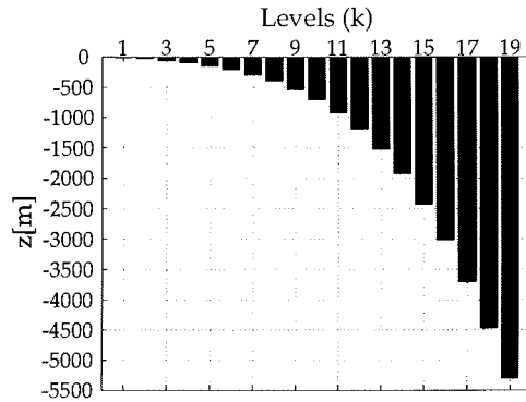
Figure 3.2: Depth levels of the scalar points, denoted as “k” in Fig. 3.1
