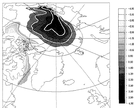
Figure 6.4: Difference of sea ice thickness between SWITCH and CTRL of the fourth year (in metres); contour interval is 1 m, values less than 0.5 m are omitted
