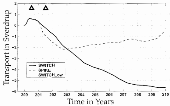
Figure 6.6: Deviation of the value of the streamfunction for the meridional overturning at 48^{\circ}\text{N} and 1500 m depth from the CTRL (in Sverdrup). The time series are filtered with a thirteen month running mean; triangles mark the switch to NAO- forcing and the return to NAO+ forcing one year later in the SPIKE experiment (compare Fig. 6.2)
