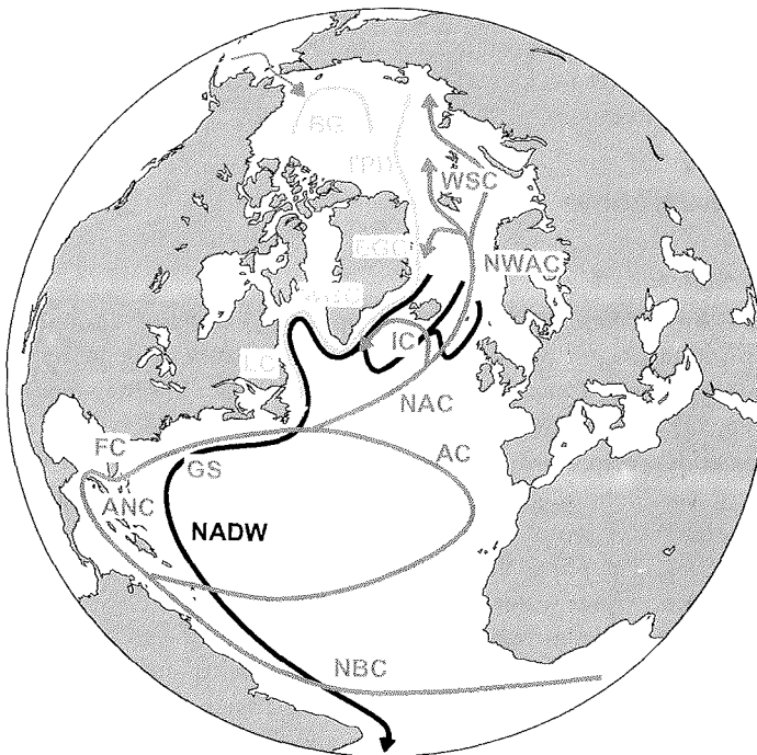
Figure 2.2: Sketch of the major currents of the North Atlantic and Arctic Ocean. Warm Currents (grey): NBC: North Brazil Current, ANC: Antilles Current, FC: Florida Current. GS: Gulf Stream, NAC: North Atlantic Current, AC: Azores Current, IC: Irminger Current, NWAC: Norwegian Atlantic Current, WSC: West Spitsbergen Current. Cold Currents (light grey): TPD: Transpolar Drift, BG: Beaufort Gyre, EGC: East Greenland Current, WGC: West Greenland Current, LS: Labrador Current. Deep Current (black): NADW: Pathway of the overflow water and North Atlantic Deep Water
