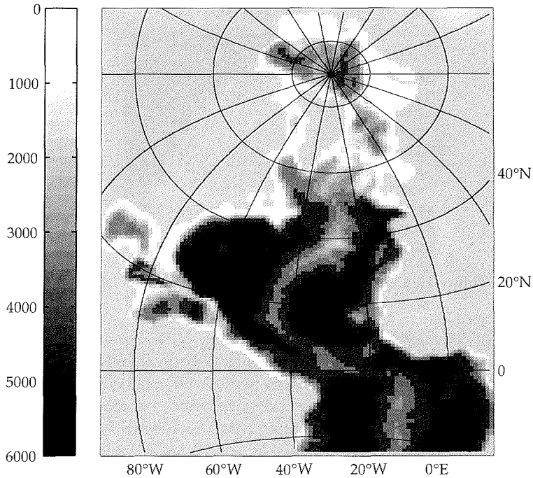
Figure 3.3: Model topography, depths in metres
