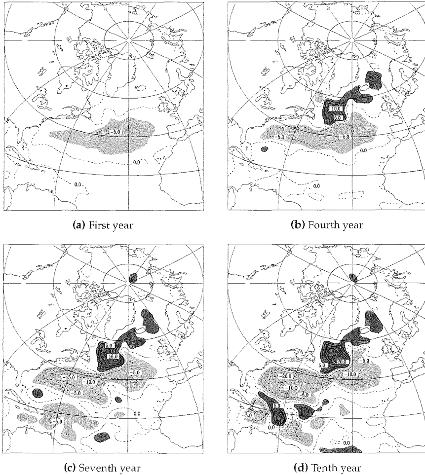
Figure 6.9: Difference between SWITCH and CTRL in the barotropic streamfunction with a contour interval of 5 Sv; values smaller than -2.5 Sv are lightly shaded, values larger than 2.5 Sv are heavily shaded
