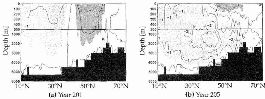
Figure 6.7: Annual mean meridional overturning of the SWITCH experiment as deviation from CTRL (in Sverdrup), values smaller than -0.5\text{ Sv} are lightly shaded, values larger than 0.5\text{ Sv} are heavily shaded
