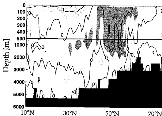
Figure 6.8: Year 205 of the annual mean meridional overturning of the SWITCH ow experiment as deviation from CTRL (in Sverdrup), values smaller than -0.5 Sv are lightly shaded, values larger than 0.5 Sv are heavily shaded
