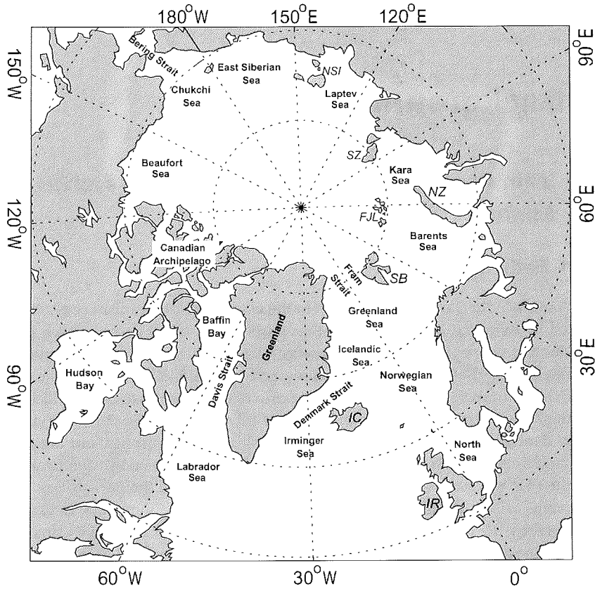
Figure 2.1: Arctic Mediterranean Sea, NZ: Novaja Zemlja, NSI: New Siberian Islands, SZ: Severnaja Zemlja, FJL: Franz-Josef-Land, SB: Svalbard, IC: Iceland, IR: Ireland
