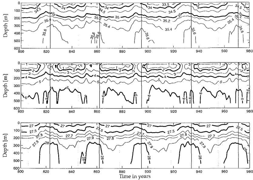
Figure 7.5: Mean layer profiles in the Labrador box as Hovmöller diagrams over time; upper panel: salinity, middle panel: potential temperature, lower panel: potential density in sigma units; the maxima of the overturning are marked with vertical grey lines, the minima with vertical dotted grey lines
