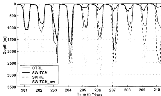
Figure 6.13: Maximal convection depth in the Labrador box (in metres)
