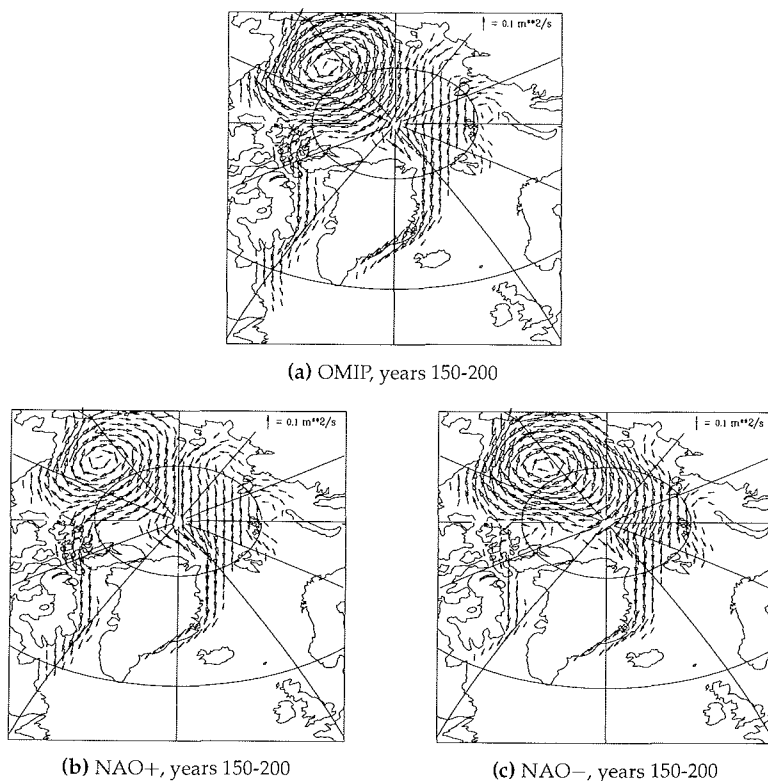
Figure 5.9: Mean ice transport averaged over year 150 to 200 (in \bar{u}h )
