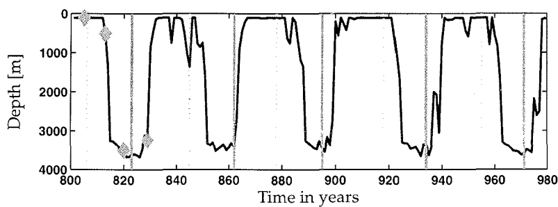
Figure 7.6: Maximal convection depth in the Labrador box in March (in metre); the diamonds mark the distinct times of four different phases of the overturning (years 805, 813, 820 and 829)
