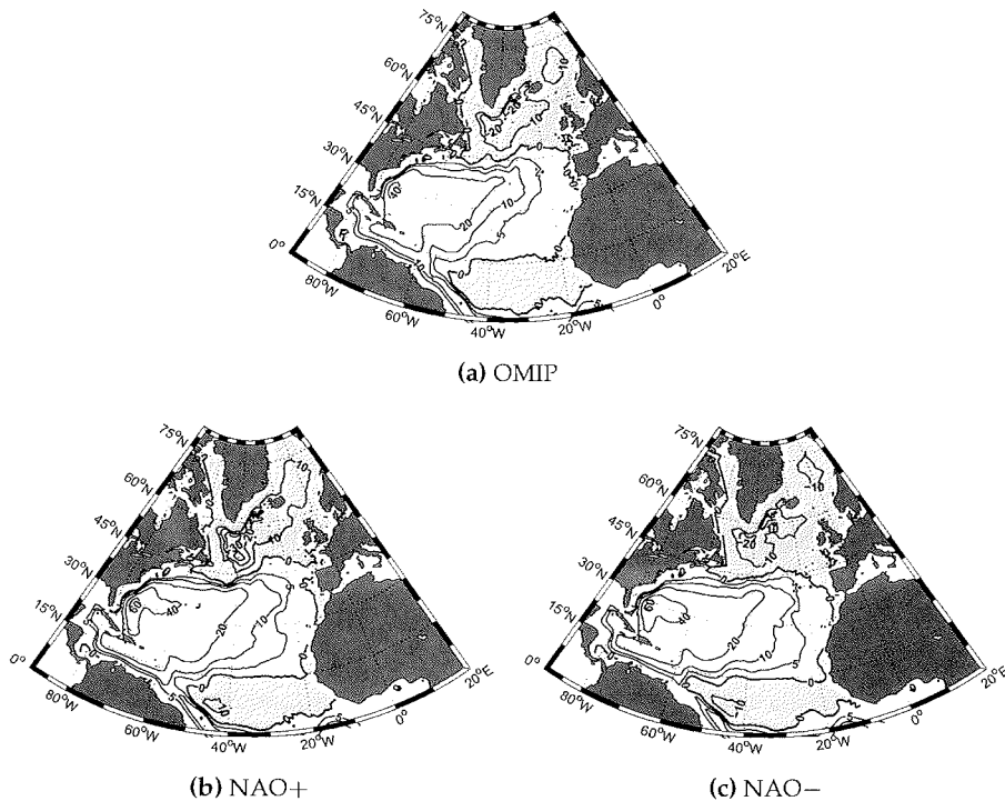
Figure 5.3: Mean vertically integrated streamfunction of the North Atlantic in Sverdrup ( 1 \text{ Sv} = 10^6 \text{ m}^3/\text{s} ), averaged over the years 150 to 200. Areas of negative values are shaded; a) 50 year mean of OMIP experiment, b) 50 year mean of NAO+ experiment and c) 50 year mean of NAO- experiment.
