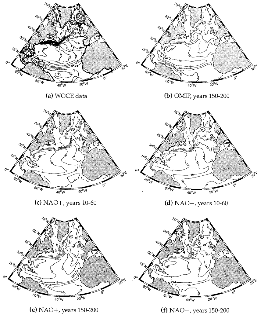
Figure 5.1: Potential temperature in 300 m depth of the North Atlantic, averaged over 50 years (in °C). a) The climatology of GOURETSKI AND JANCKE (1998), b) OMIP experiment, mean of years 150-200, c) NAO+ experiment mean of years 10-60, d) NAO- experiment, mean of years 10-60, e) NAO+ experiment mean of years 150-200, f) NAO- experiment, mean of years 150-200.
