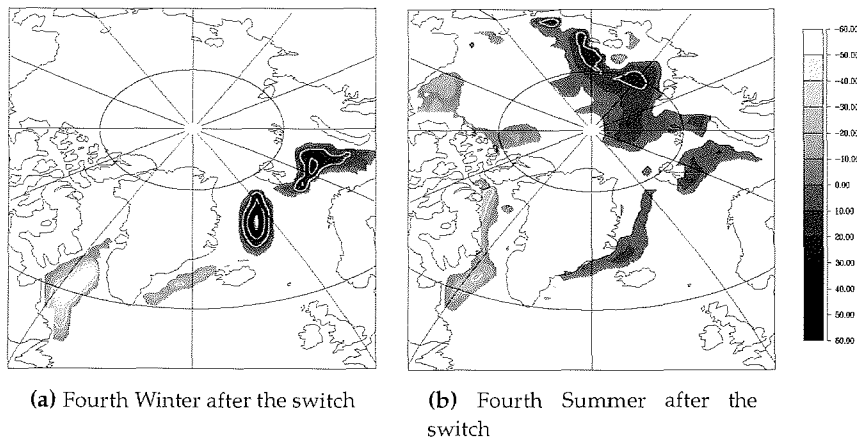
Figure 6.3: Difference of sea ice concentration between SWITCH and CTRL (in percent); contour interval is 20%, values less than 5% are omitted
