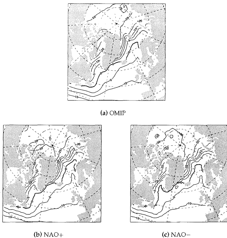
Figure 4.2: NDJFMA mean of the surface air temperature (in °C); a) OMIP year, b) NAO+ composite, c) NAO- composite
