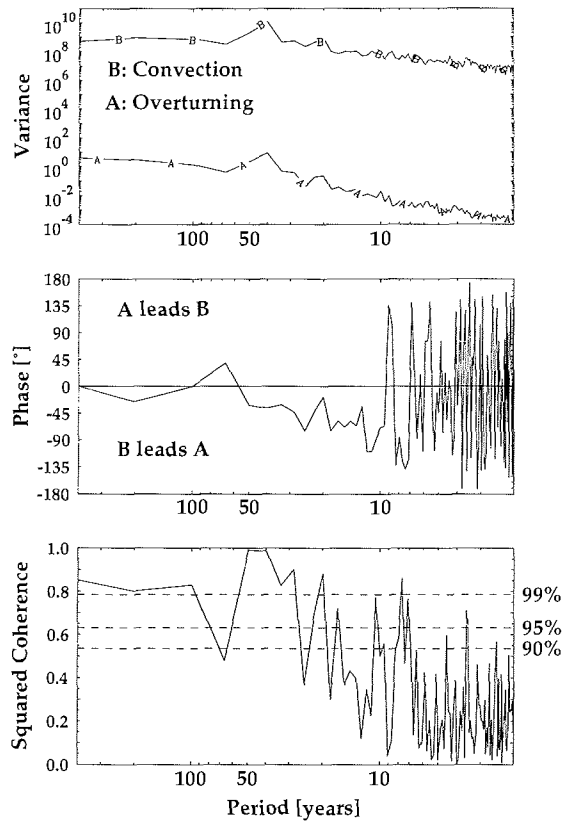
Figure 7.8: The cross-spectra of the maximum of the overturning streamfunction (A) and the maximum of the convection in March in the Labrador box (B). Top panel: spectral variance; middle panel: phase spectrum, lower panel: squared coherency; the significance of the squared coherency is estimated by a Bartlett procedure with a chunk length of 200 years
