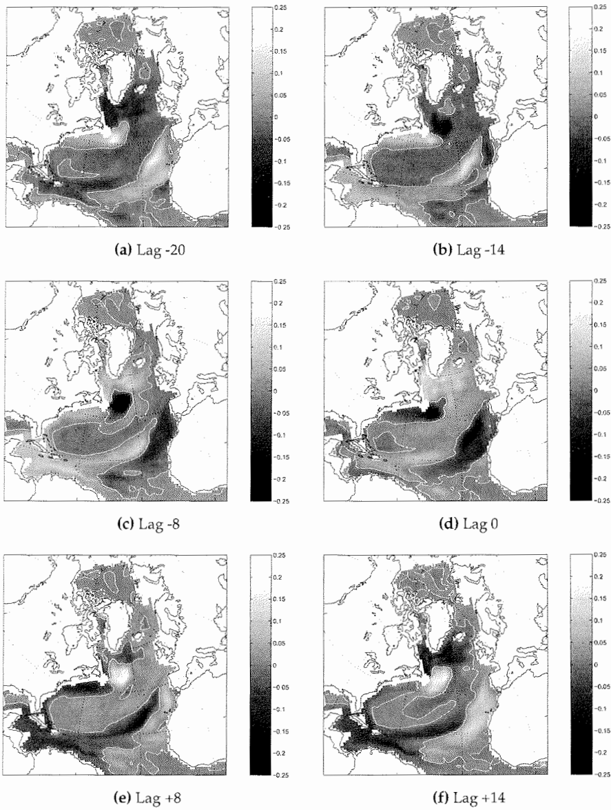
Figure 7.7: Associated patterns of the maximum of the overturning and salinity at 300 m depths for specific lags, the white line corresponds to zero
