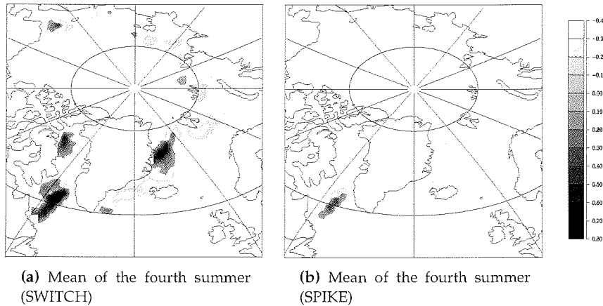
Figure 6.5: Difference of sea ice growth of SWITCH and SPIKE, relative to CTRL (in metres/month); values less than \pm 0.1 metres/month are omitted
