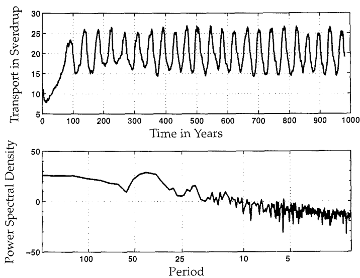
Figure 7.1: Time series of the oscillation; upper panel: meridional overturning at 48°N and 1500 m depth; lower panel: spectrum of the time series
