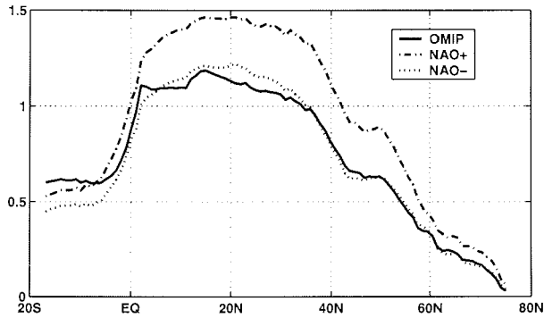
Figure 5.6: Northward heat transport as a mean over year 150 to 200 (in Petawatt, 1 \text{ PW} = 10^{15} \text{ W} ).
