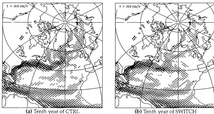
Figure 6.10: Annual mean velocity field in 100 m depth (in cm/s); values less than 1.0 cm/s are cut off, quadratic scale of arrow length
