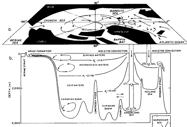
Figure 2.3: Schematic circulation and water mass structure in the Arctic Mediterranean from AAGAARD ET AL. (1985)
