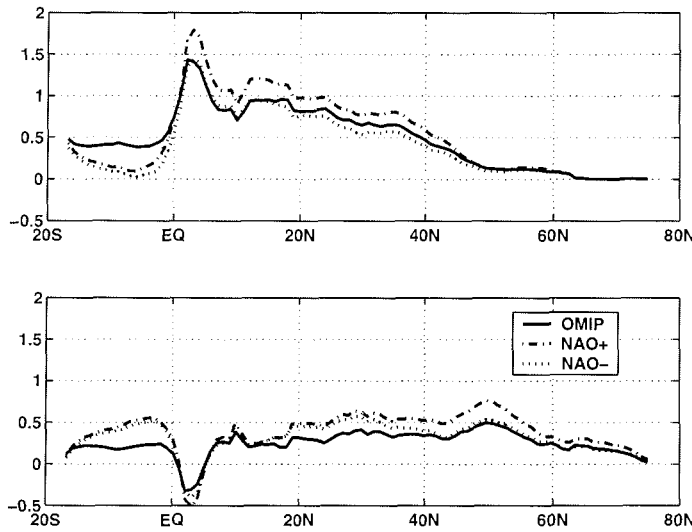
Figure 5.7: Decomposition of the northward heat transport as a mean over year 150 to 200 (in Petawatt); the upper panel shows the overturning component, the lower panel the gyre component of the total advective heat transport
