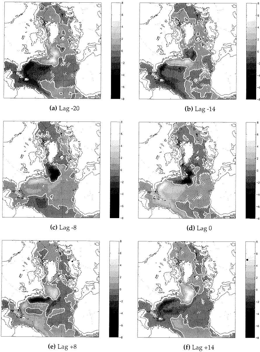
Figure 7.2: Associated patterns of the streamfunction for the vertically integrated transport regressed upon the overturning index defined as the value of the overturning streamfunction at 48N and 1500m depth. The white line corresponds to zero. Lags are given in years relative to the maximum of the overturning where negative lags mean that the streamfunction anomalies lag behind the overturning
