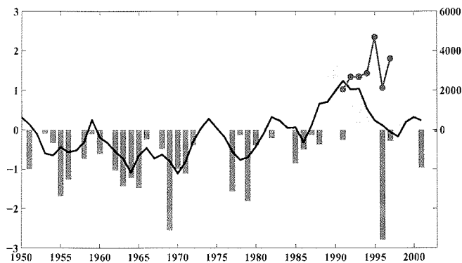
Figure 6.1: NAO Index (Dec - Mar): SLP difference Gibraltar-Stykkisholmur as defined by JONES ET AL. (1997) (updated); the black line is the running mean over five years; the grey dots denotes the ice export through Fram Strait as measured by VINJE ET AL. (1998) (in \text{km}^3/\text{yr} )
