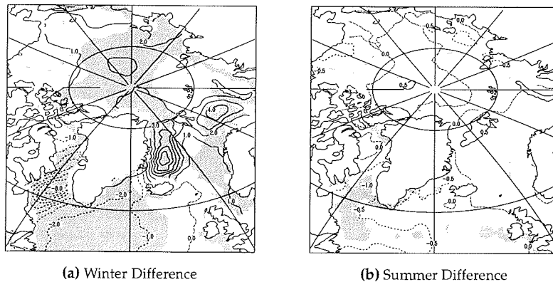
Figure 4.4: Difference between the NAO+ and NAO- composite of the two metre temperature in °C (significant regions are shaded)
