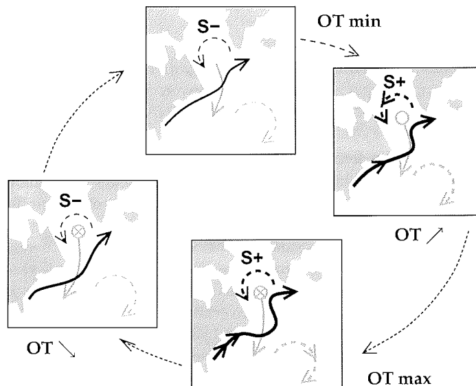
Figure 7.12: Sketch of an oscillation cycle; the black line indicates the pathway and strength of the NAC; the grey line the pathway and strength of the DWBC; grey circle and cross stand for mid-depth and deep convection; the dashed grey line denotes the strength of the subtropical gyre, the dashed black line the strength of the subpolar gyre; S- ( S+ ) is a negative (positive) salinity anomaly
