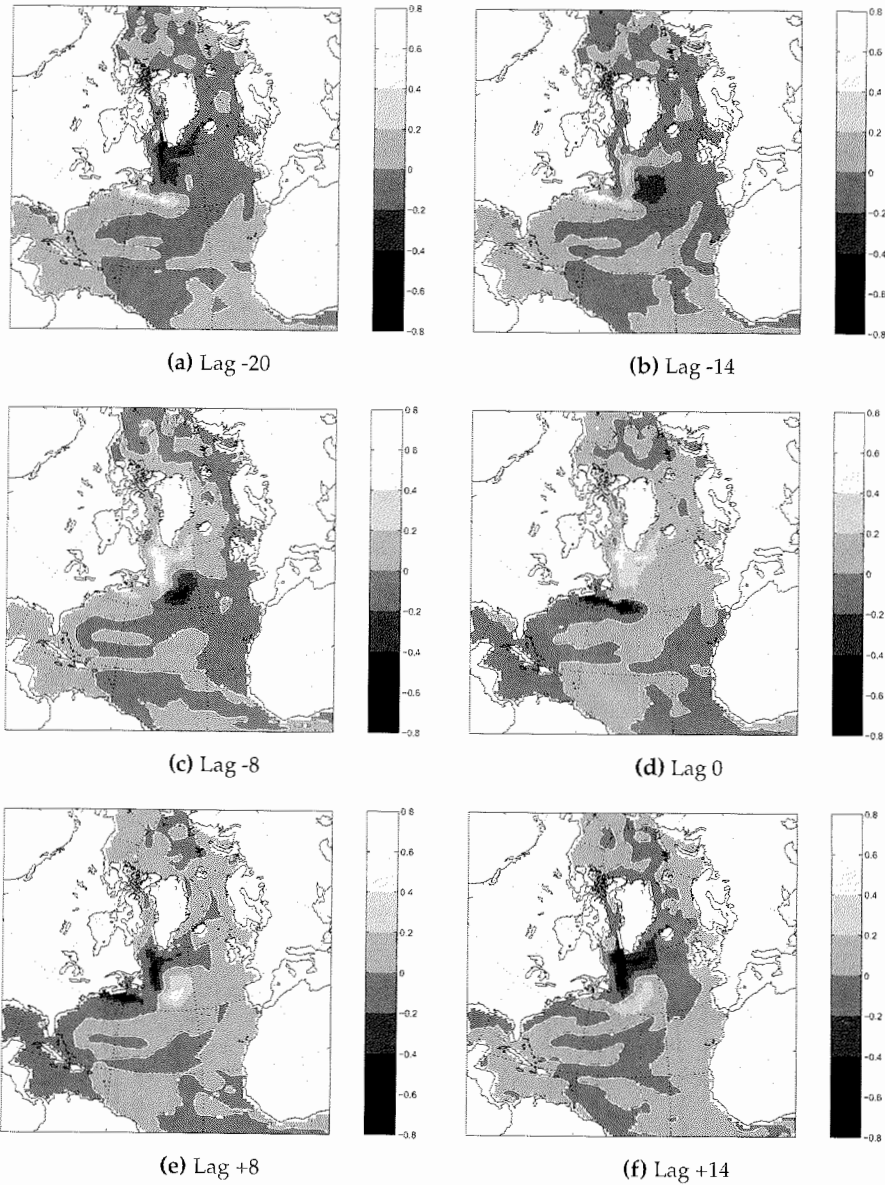
Figure 7.4: Associated patterns of the maximum of the overturning and sea surface salinity (SSS) for specific lags, the white line corresponds to zero
