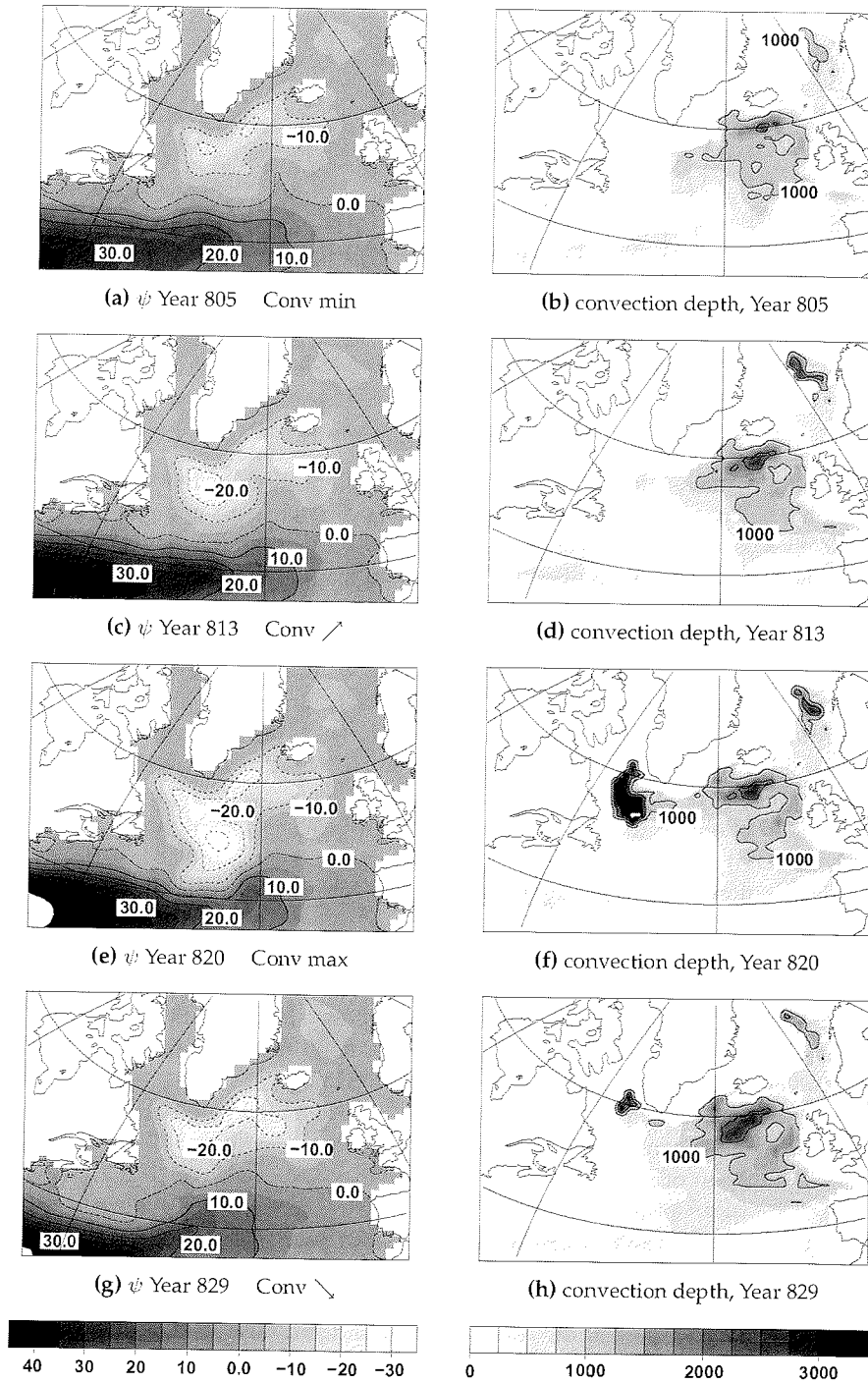
Figure 7.10: Annual means of the streamfunction (in Sv) and convection depths (in metres) in the northern North Atlantic for distinct years, only convection depths larger than 100 m are shown
