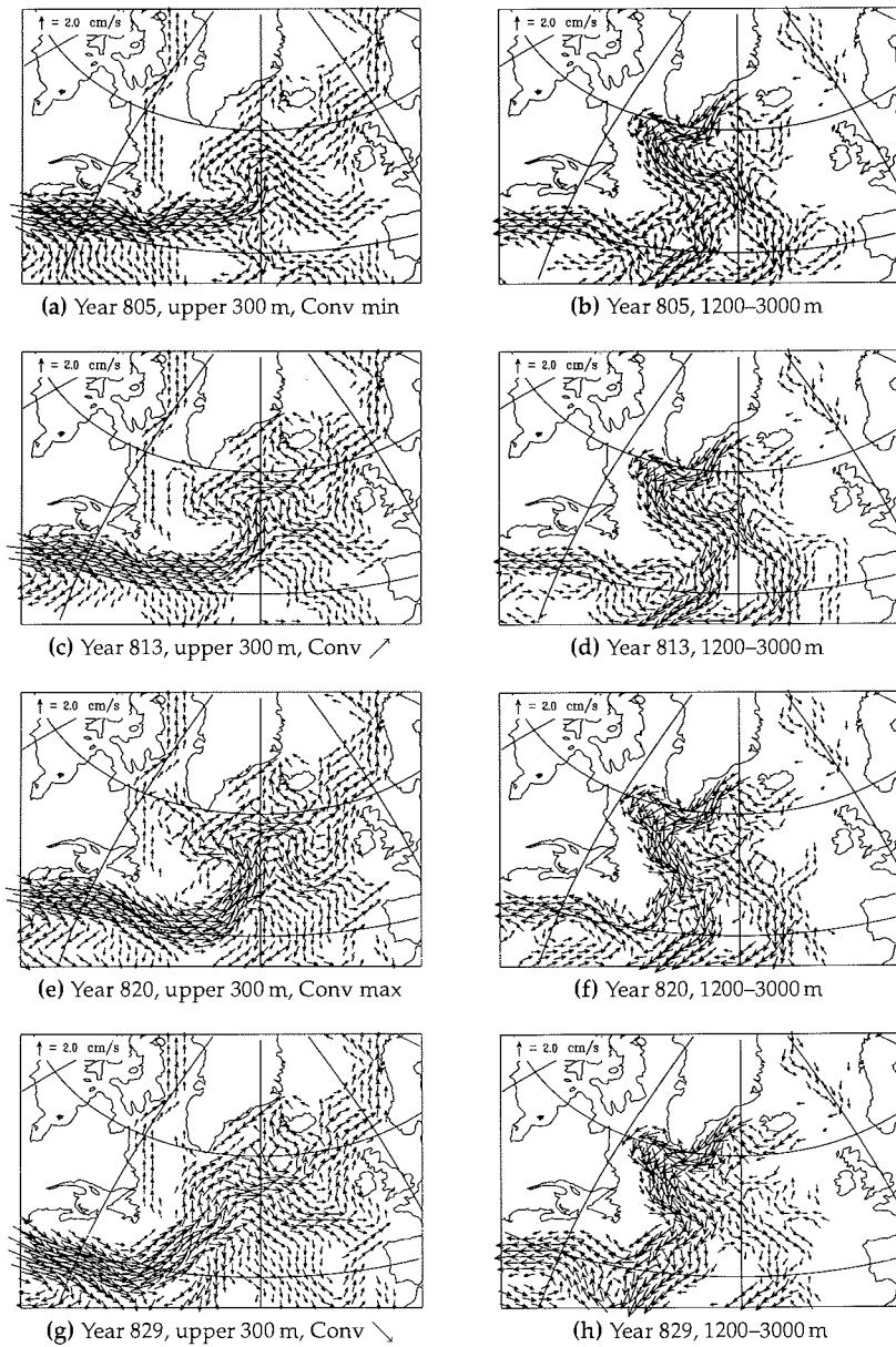
Figure 7.11: Annual means of salt transport relative to 34.46 in the northern North Atlantic for the upper 300 m and for the depth of the DWBC (1200-3000 m)
