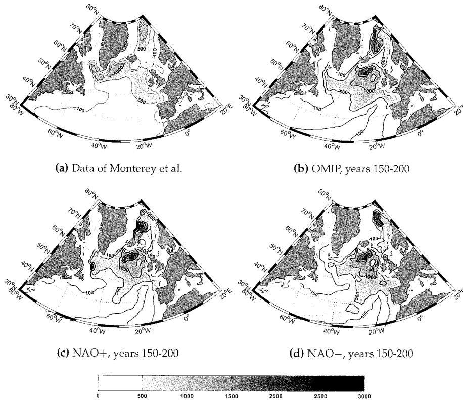
Figure 5.4: Mean mixed layer depth in March, averaged over years 150 to 200 (in metres); a) Climatology of March of MONTEREY AND LEVITUS (1997), b) 50 year mean of OMIP experiment, c) 50 year mean of NAO+ experiment and c) 50 year mean of NAO- experiment.
