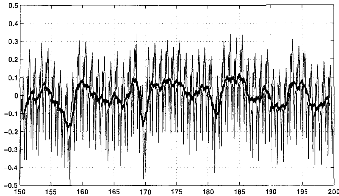
Figure 5.8: Anomaly of the northward heat transport of NAO– for the years 150 to 200 as monthly means at 20°N (in Petawatt); the thick line is a running mean over 13 months
