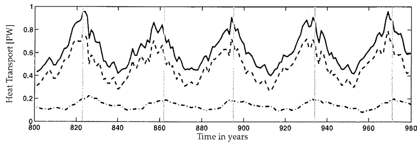
Figure 7.3: Fluctuations of the meridional heat transport at 48°N (solid black line) and its decomposition in gyre (dashed line) and overturning component (dashed-dotted line); the maxima of the overturning are marked with vertical grey lines, the minima with vertical dotted grey lines
