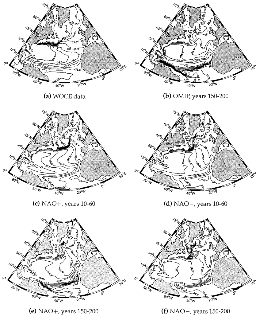
Figure 5.2: Salinity in 300 m depth of the North Atlantic, averaged over 50 years. a) The climatology of GOURETSKI AND JANCKE (1998), b) OMIP experiment, mean of years 150-200, c) NAO+ experiment mean of years 10-60, d) NAO- experiment, mean of years 10-60, e) NAO+ experiment mean of years 150-200, d) NAO- experiment, mean of years 150-200.
