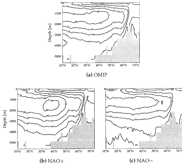
Figure 5.5: Mean zonally integrated overturning streamfunction of the North Atlantic, averaged over years 150 to 200 (in Sverdrup). a) 50 year mean of OMIP experiment, b) 50 year mean of NAO+ experiment, c) 50 year mean of NAO- experiment.
