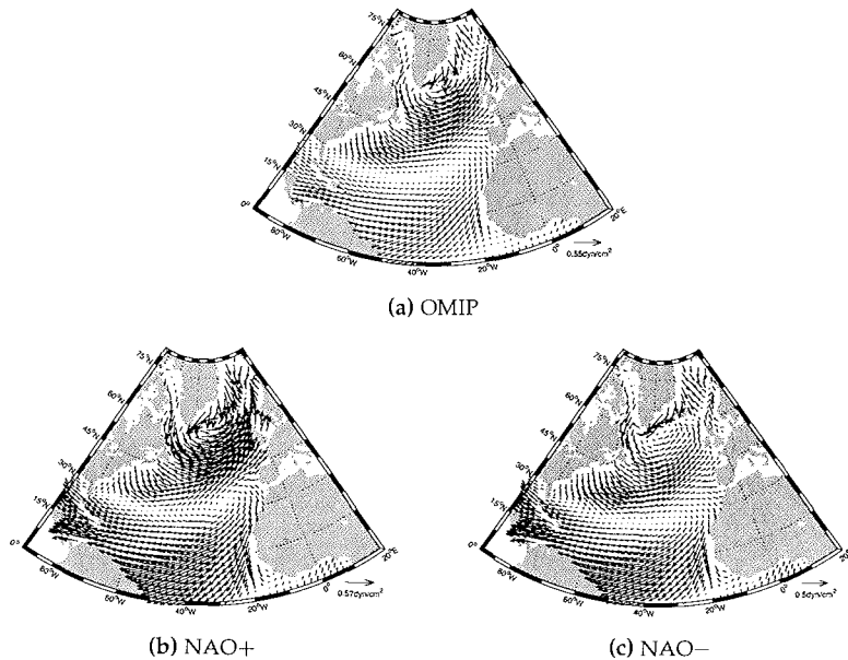
Figure 4.1: NDJFMA mean of the windstress fields (in \text{dyn}/\text{cm}^2 ); a) OMIP year, b) NAO+ composite, c) NAO- composite
