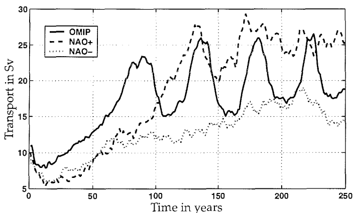
Figure 5.10: Annual mean of the maximum of the meridional overturning at 48^{\circ}\text{N} and 1500 m depth for 250 years of the three experiments (in Sverdrup)
