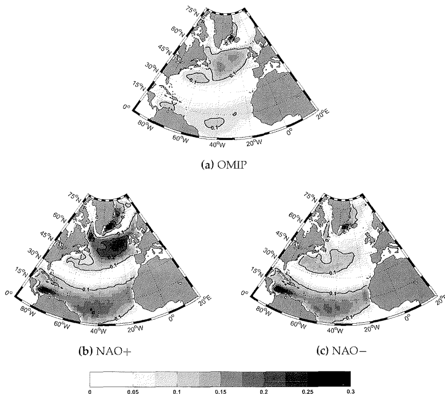
Figure 4.5: NDJFMA mean of the magnitude of the wind stress vector (in N/m^2 ); a) OMIP year, b) NAO+ composite, c) NAO- composite
