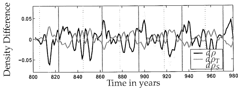
Figure 7.9: Temporal derivatives of density difference between the upper 300 m and the adjacent 300 m, based on yearly mean values; separated into the salinity \rho_S and temperature \rho_T parts of the density difference
