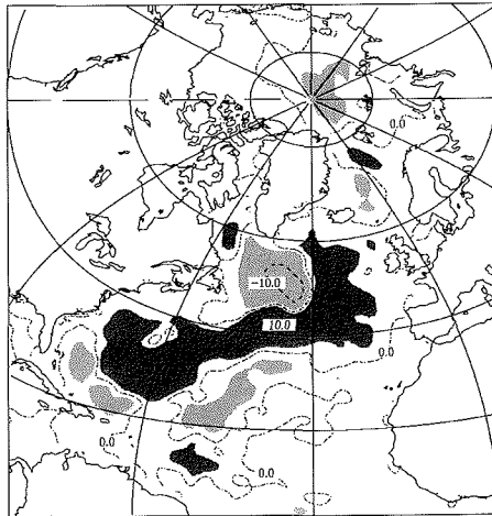
Figure 6.12: Annual mean of the integrated potential energy anomaly for the tenth year of SWITCH ow in Sverdrup; figure caption as in Fig. 6.11
