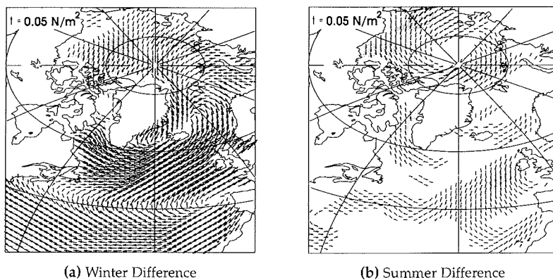
Figure 4.3: Difference between the NAO+ and NAO- composite of the wind stress (in N/m^2 ; significant regions are the shades; quadratic scale of arrow length)
