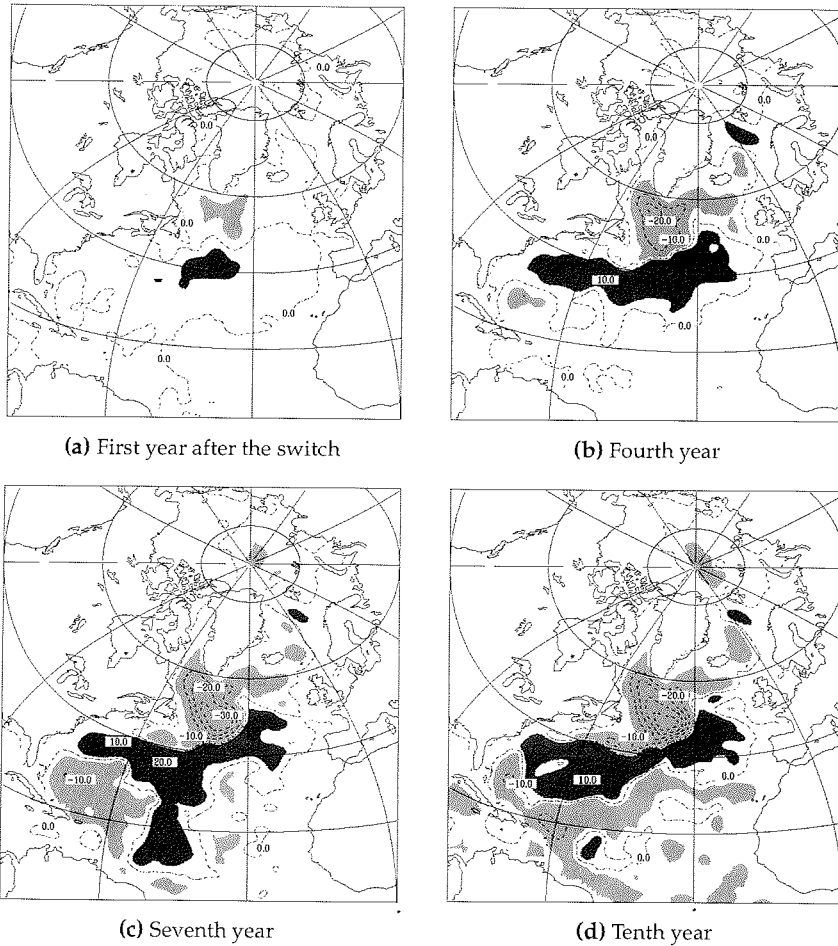
Figure 6.11: Annual means of the integrated potential energy anomaly ( \delta\chi/f_0 , where f_0 = 2\Omega\sin(50^\circ) ) of SWITCH versus CTRL in Sverdrup (compare Eq. (6.2)); contour interval is 10 Sv; values smaller than -5 Sv are lightly shaded, values larger than 5 Sv are heavily shaded
