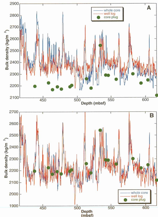
Fig. 5 - Comparison of three suites of bulk density measurements: whole-core (Cape Roberts Science Team, 2000), well logs calibrated to whole-core data (Bucker et al., this volume), and core plugs of this study. Top: before recalibration to core plugs; bottom: after recalibration. For clarity, only a 200-m interval of the 939-m CRP-3 drillhole is shown.
