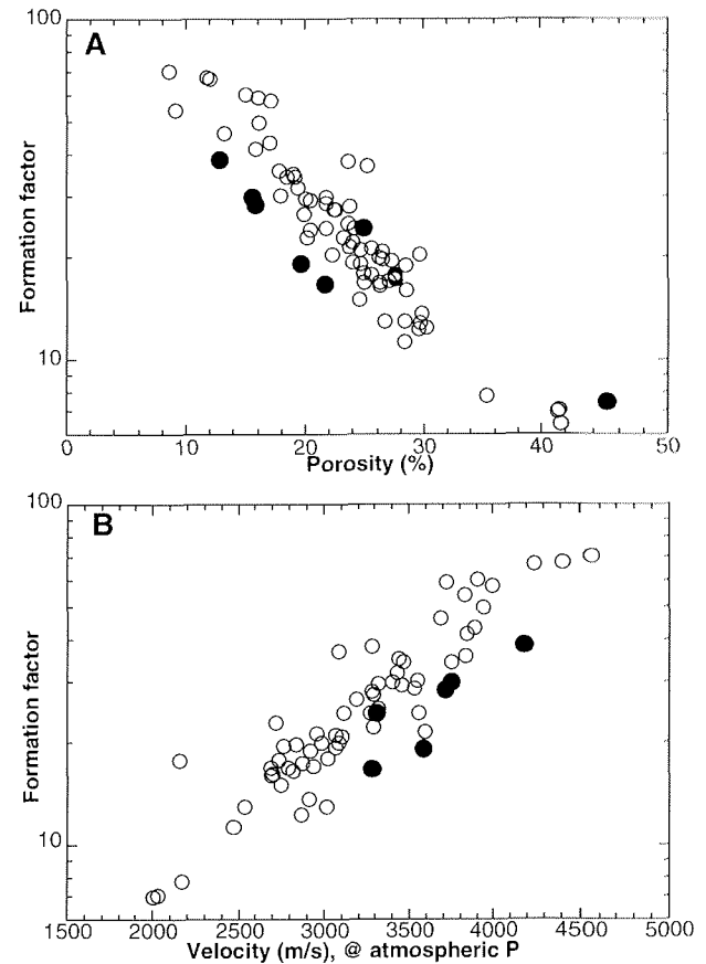
Fig. 1 - A: Relationship between formation factor and porosity. B: Relationship between formation factor and velocity. Open circles: Tertiary shelf samples; solid dots: Devonian Beacon samples.
