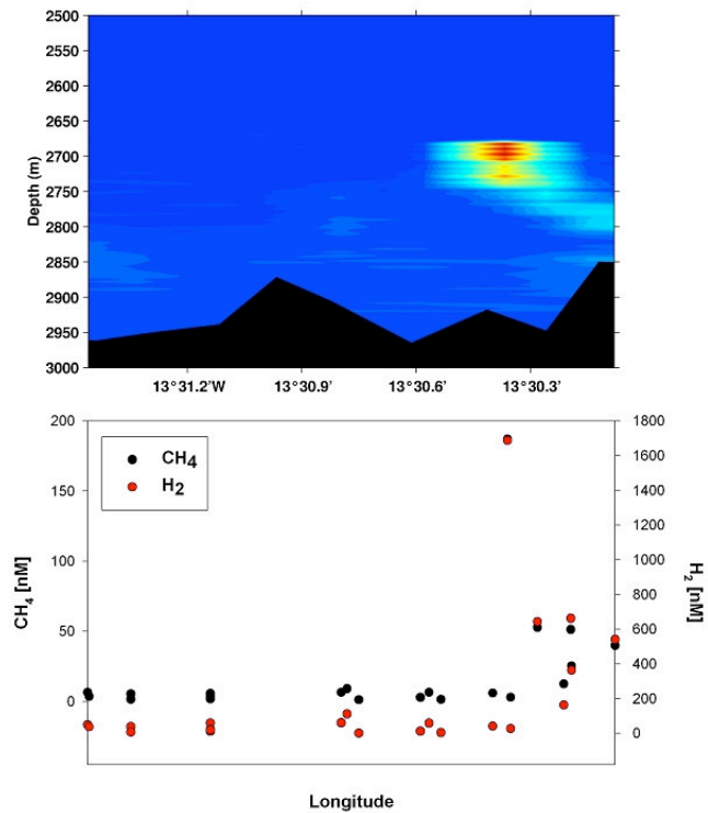
Fig. 1.44: Tow-yo (64CTD) from east to west across the “Drachenschlund” vent at 13°30.4’W. Upper section shows turbidity anomaly. The lower diagram shows methane and hydrogen concentrations of the discrete water samples as a function of position.
