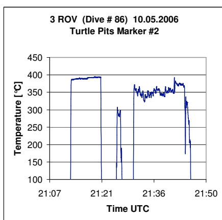
Fig. 1.49: Measured in-situ temperatures during fluid sampling with KIPS at Marker #2 Vent , Turtle Pits, in an orifice approx. 1 m above ground. Maximum temperature measured was 395.1 °C (note unstable temperature readings, compare to Fig.1.53), at a water depth of 2986 m. Samples 3 ROV-10 and -11 were taken from 21:30 – 21:45 UTC.
