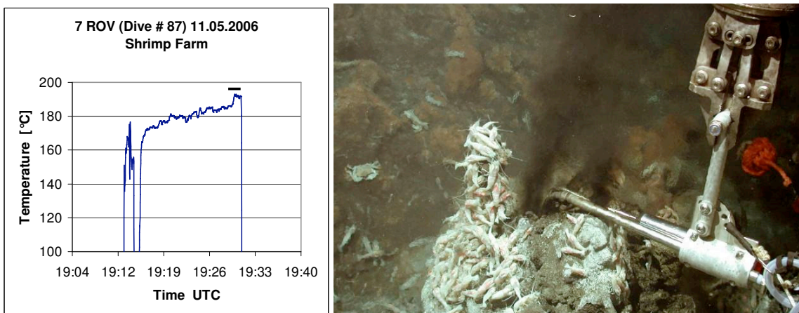
Fig. 1.51: Measured in-situ temperatures during fluid sampling with KIPS at Shrimp Farm Vent , Red Lion, orifice on top of the flange structure. Maximum temperature measured was 193.0 °C, at a water depth of 2986 m. Samples 7 ROV-1 to -3 were taken from 19:16 – 19:30 UTC.
