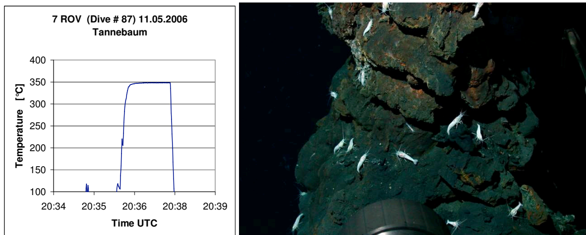
Fig. 1.52: Measured in-situ temperatures at Tannebaum Vent , Red Lion, orifice on top of the chimney. Maximum temperature measured was 349.0 °C, at a water depth of 3044 m. No samples were taken.
