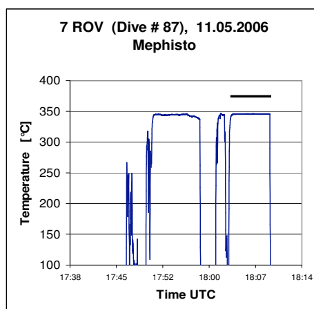
Fig. 1.50: Measured in-situ temperatures during fluid sampling with KIPS at Mephisto Ven , Red Lion, orifice on top of the chimney. Maximum temperature measured was 346.3 °C, at a water depth of 3098 m. Samples 7 ROV-1 to -3 were taken from 7:50 – 18:08 UTC.
