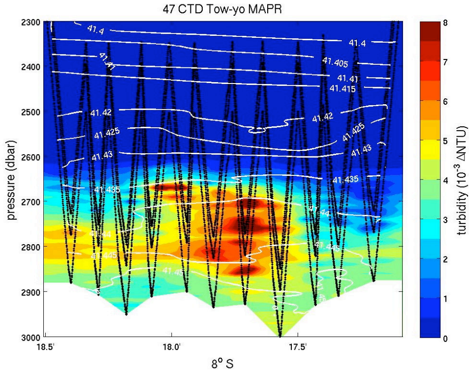
Fig. 1.37: Turbidity anomaly along a Tow-yo track with CTD and MAPR (Miniature Autonomous Plume Recorder) across the plume dispersion in S-N direction in the Nibelungen field.
