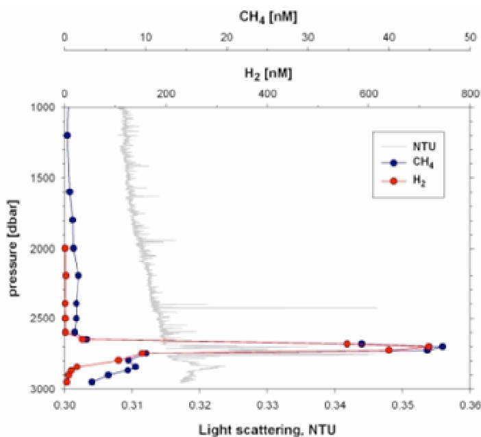
Fig. 1.43: Methane, hydrogen and optical backscatter at Station 43CTD (8°17.9'S, 13°30.7'W).
