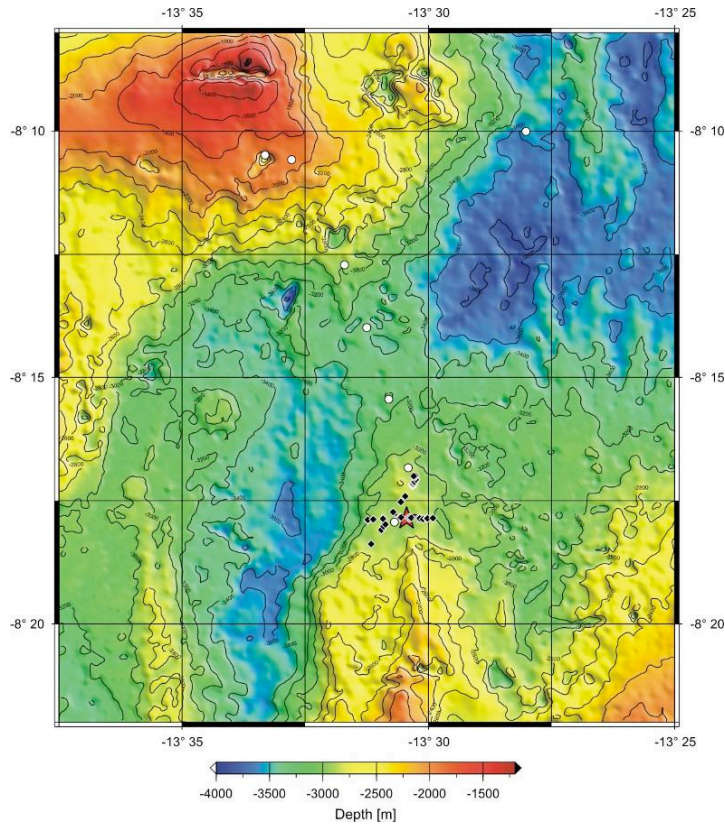
Fig. 1.36: Map of the 8°S working area. Red stars denote the vent sites, white dots classical CTD/LADCP stations and black diamonds water samples during tow-yo casts. Map by O. Schmale.
