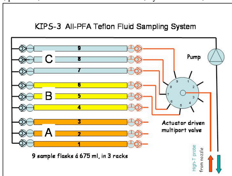
Fig. 1.47: Schematic configuration of the inert KIPS fluid sampling system (only tubing connections to flasks # 5 - # 9 are shown for clarity). Fluid entering the nozzle is distributed by a motorized multiport-valve to 9 PFA sample flasks of 675 ml, each with check valves and stopcocks. The pump is positioned downstream. Racks A, B, C with 3 flasks each can be quickly removed and sub-sampled in the lab.
