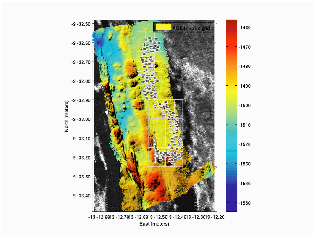
Fig. 1.21: TOBI-side scan imagery, ABE SM2000 bathymetry and ROV-based seafloor observations in the area of the Lilliput hydrothermal field.
