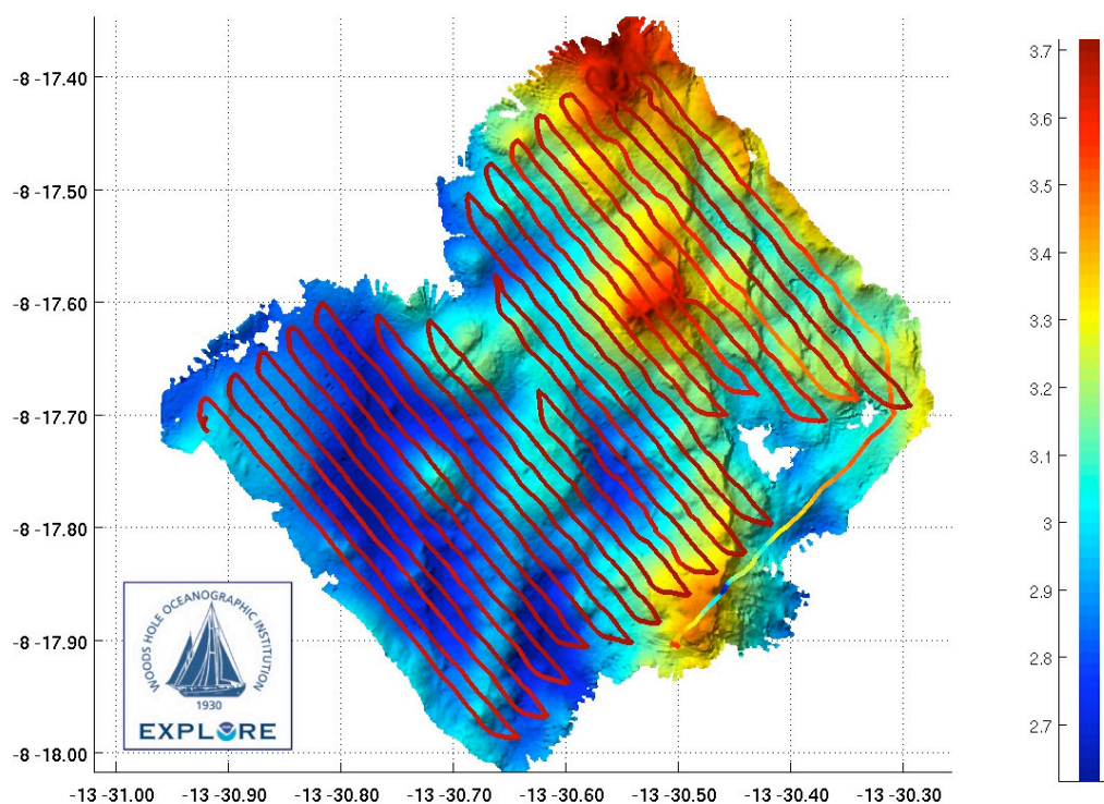
Fig 1.6: Eh data superimposed on the multibeam bathymetry for the ABE178 dive.
