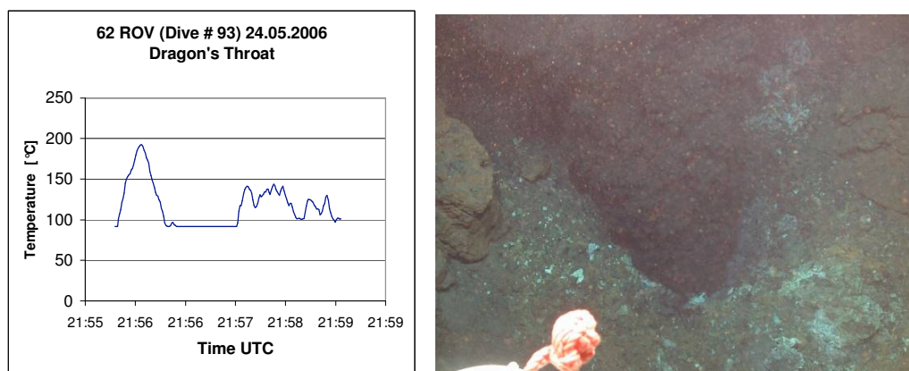
Fig. 1.56: Measured in-situ temperatures at Dragon's Throats , but nozzle could not be correctly inserted into orifice. Maximum temperature measured was 192 °C, at a water depth of 2910 m. Samples 62 ROV-5 and -9/-10 taken from 20:08 until 20:18 UTC.
