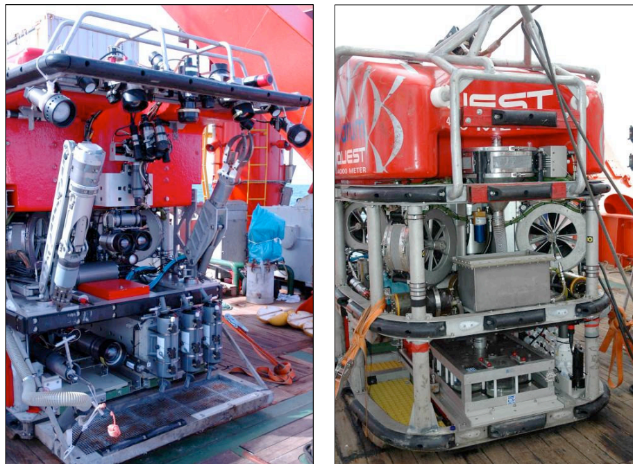
Fig. 1.9, left: “QUEST4000m” front view (from top to bottom): upper porch with lights, strobes, sonar, beacon finder, InsitePacific AURORAs, and USBL transducers; upper pan&tilt with light, DSPL Seacam6500, and lasers; lower pan&tilt with InsitePacific PEGASUS and SCORPIO, and light; Orion manipulator on left, Rigmaster manipulator on right; two forward lateral thrusters (FS, FP) on behind; on toolskid from left to right suction hose for rotary sampler, KIPS fluid sampling nozzle and high temperature sensor, InsitePacific ATLAS, tool/sample box with three Niskin bottles; lower porch with grating
