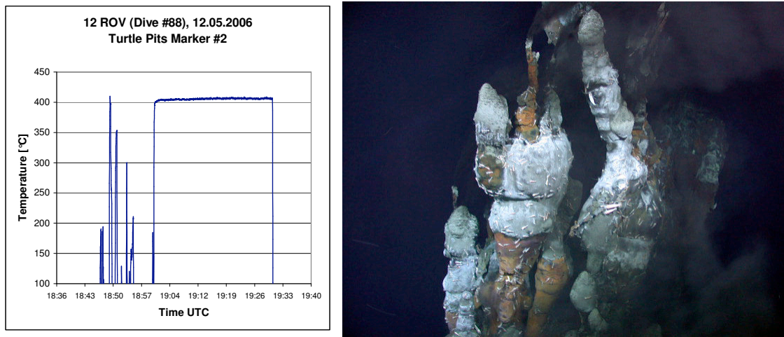
Fig. 1.53: Measured in-situ temperatures during fluid sampling with KIPS at Marker #2 Vent , Turtle Pits in the same orifice approx. 1 m above ground already sampled during 3 ROV. Maximum temperature measured was 408.7 °C, at a water depth of 2988 m. Samples 12 ROV-4 to -8 were taken from 19:01 – 19:30 UTC.
