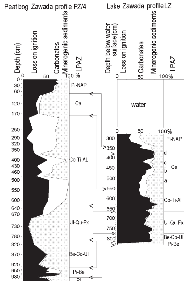
Fig. 10. Main sediment components of the Lake Zawada and peat bog Zawada 4: loss on ignition, \text{CaCO}_3 content in the ignition residue and minerogenic sediment
