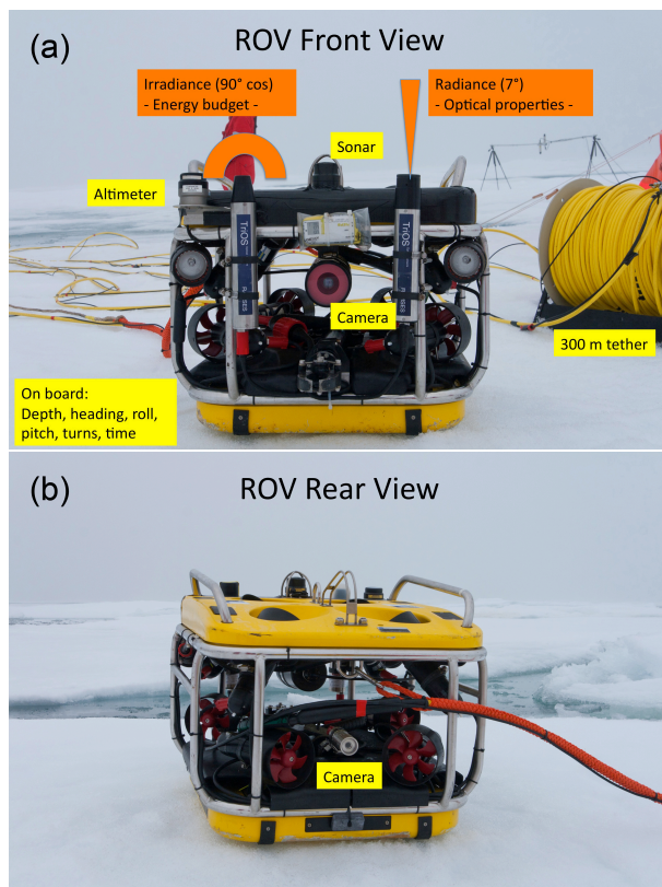
Fig. 2. Annotated photographs of the ROV equipped with sensors for under-ice radiation measurements. (a) Front view including the two Ramseys radiometers, one measuring irradiance (left) and one measuring radiance (right). Surface sensors are shown in the back, too. (b) Rear view with tether.
