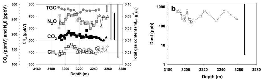
Figure 3. Gas and dust properties of the deep (squares) and basal (triangles) ice at EPICA Dome C: (a) total gas content ( \text{ml}_{\text{air}} \text{g}_{\text{ice}}^{-1} , dark grey), methane (ppbV, white), nitrous oxide (ppbV, light grey) and carbon dioxide (ppmV, black) – vertical bars of equivalent shading cover the full concentrations range observed for \text{CH}_4 , \text{CO}_2 , \text{N}_2\text{O} and total gas content during the preceding climatic cycles, (b) dust concentrations (ppb) – black vertical bar covers the full concentration range during the previous climatic cycles.
