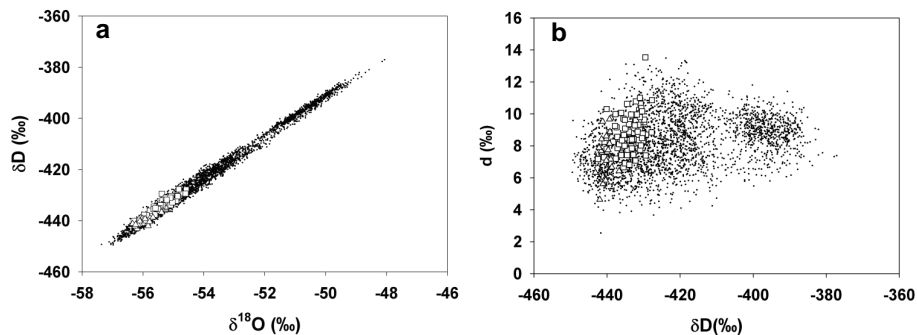
Figure 2. (a) \delta D_{\text{ice}} (‰) vs. \delta^{18}O_{\text{ice}} (‰) and (b) d (deuterium excess ‰) vs. \delta D_{\text{ice}} (‰) for the deep (open squares) and basal (open triangles) ice at EPICA Dome C, as compared to the ice from the 0–140 ky interval (black dots, Stenni et al., 2010). See text for details.
