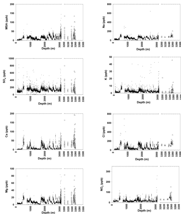
Figure 4. Concentrations (in ppb or ngg -1 ) of selected chemical species in the deep (open squares) and basal (open triangles) ice of the EPICA Dome C core, as compared to those of the preceding climatic cycles (black dots, courtesy of the EPICA chemical consortium). Resolution is between 5 and 8 cm above 3200 m depth and between 1.5 and 5 cm in the deep and basal ice below 3200 m. Note the change of depth scale below 3200 m.
