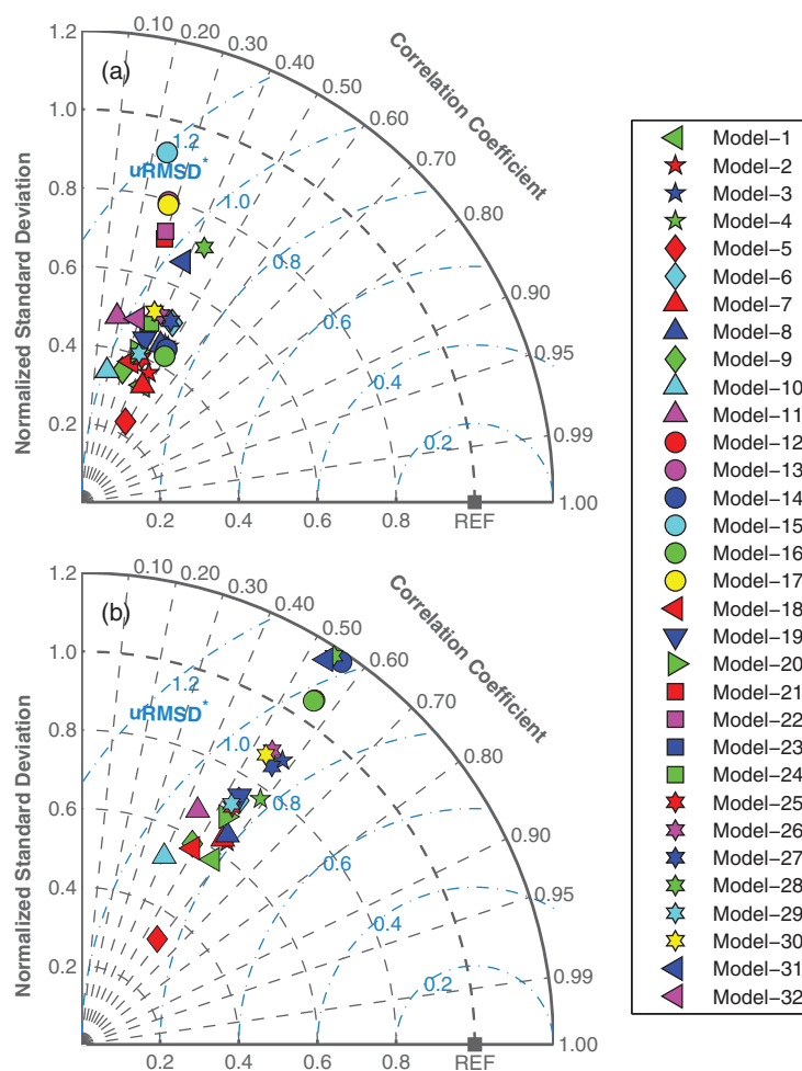
Figure 7. Taylor diagrams illustrating relative model performance in reproducing \log NPP_{N=85} using (a) satellite chlorophyll (Case 1) and (b) in situ chlorophyll (Case 9). The black square labeled as “REF” represents a perfect model, where the normalized standard deviation and the correlation coefficient are 1.0.
