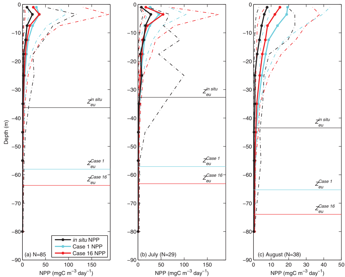
Figure 12. Vertical profiles of the mean in situ (black) NPP and the mean NPP of the 11 depth-resolved models (Models 1–8, 12, 14, and 16) in (a) all months (N=85), (b) July (N=29), and (c) August (N=38): Case 1 NPP (blue) and Case 16 NPP (red) with the averaged confidence interval of 1 standard deviation (dotted lines). NPP was grouped and averaged at given depth layers: 0–2 m, 2–5 m, 5–10 m, 10–15 m, 15–20 m, 20–30 m, 30–40 m, 40–50 m, 50–60 m, and 60–100 m. The average in situ and model Z_{eu} (Case 1 and 16) are also shown.
