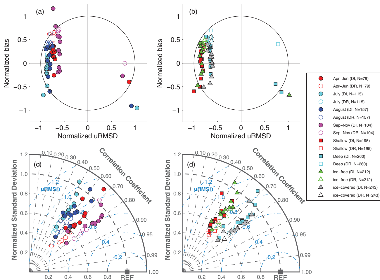
Figure 14. (a, b) Target and (c, d) Taylor diagrams of Case 16 (N=455) using in situ chlorophyll (1988–2011), illustrating relative model performance in reproducing logNPP over different (left) months and (right) regions. The symbols indicate the statistics between in situ and estimated logNPP in four different periods (April–June, July, August, and September–November), two different regions (shallow-water stations where water depth is less than 200 m and deep stations where water depth is greater than 200 m), two different sea ice conditions (ice-free stations where sea ice concentration was less than 15% and ice-covered stations where sea ice concentration was greater than 15%), and two different model types (5 depth-resolved (DR) and 11 depth-integrated (DI) models). See text for further details.
