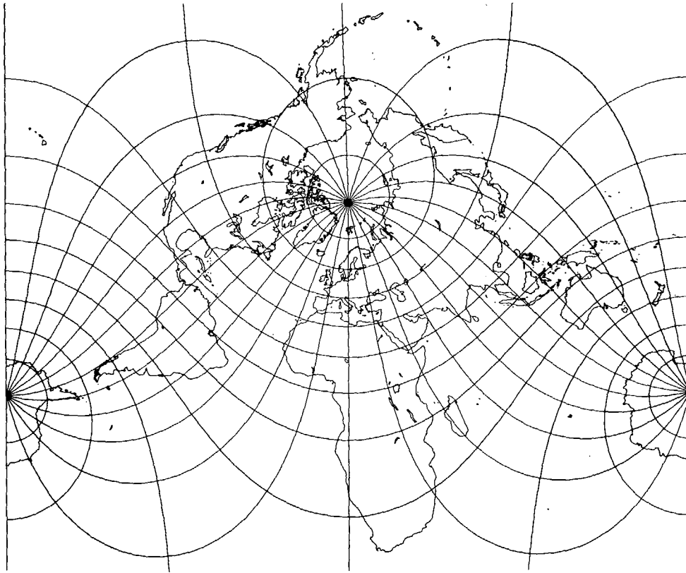
FIGURE 12.—Oblique Mercator projection with the center of projection at lat. 45° N. on the central meridian. A straight line through the point and, in this example, perpendicular to the central meridian is true to scale. The projection is conformal and has been used for regions lying along a line oblique to meridians.
