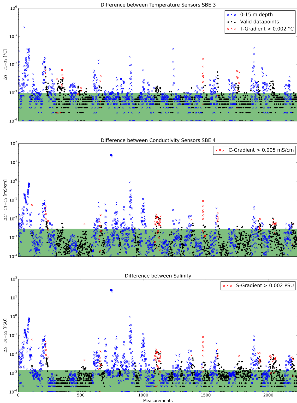
Figure 2: Data accuracy of sensor pairs HE440
