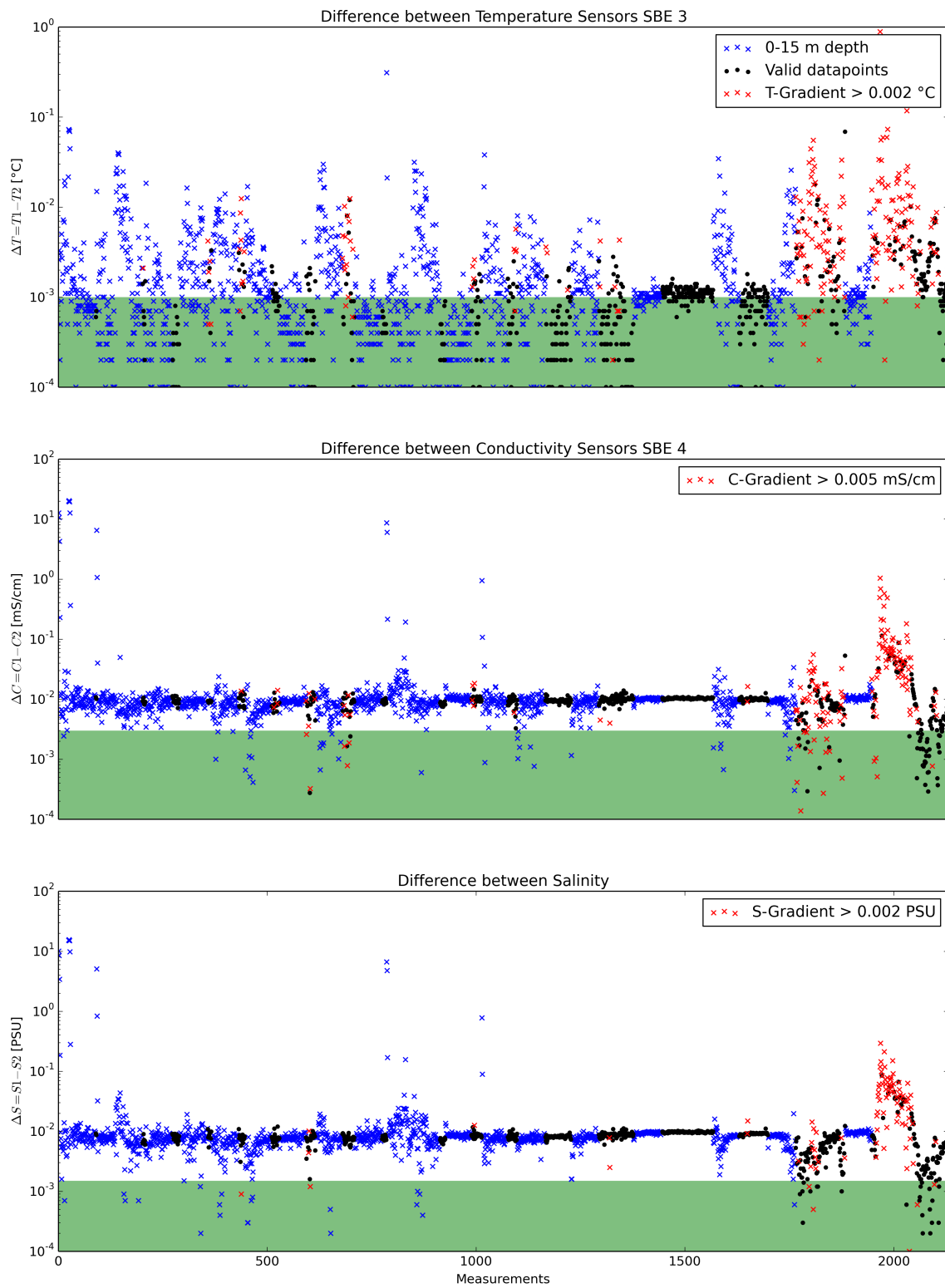
Figure 2: Data accuracy of sensor pairs HE430
