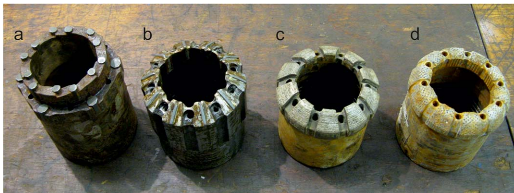
Figure 3. MeBo70 drill bits used during PS104: (a) two step tungsten carbide bit, (b) conical tungsten carbide bit, (c) diamond-impregnated bit, and (d) surface-set diamond bit.
