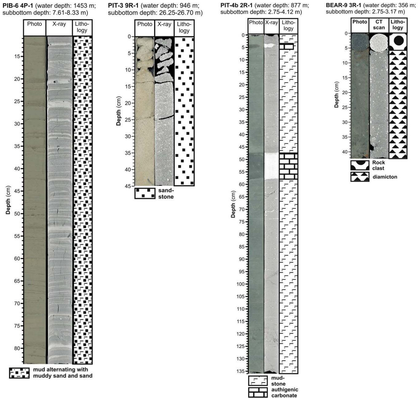
Figure 6. Examples of photo, X-radiograph, and lithology records of some of the drill cores. For lithological key, see Figure 7.
