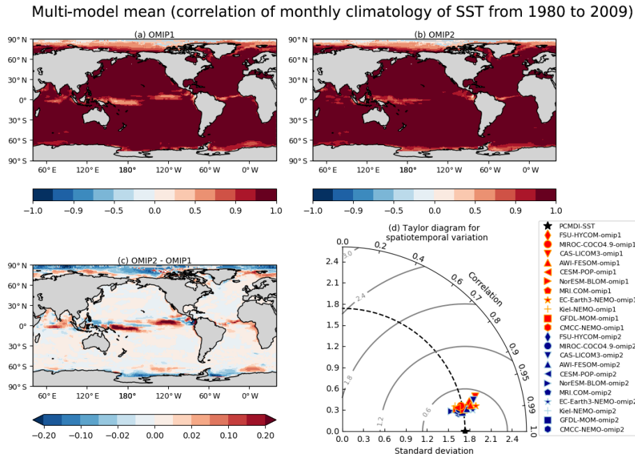
Figure E1. Multi-model mean correlation coefficients of monthly climatology of SST for the period 1980–2009 between simulation and PCMDI-SST. (a) OMIP-1, (b) OMIP-2, (c) OMIP-2 – OMIP-1. (d) Taylor diagram of the total space–time pattern variability of the monthly climatology of SST of OMIP-1 and OMIP-2 simulations relative to PCMDI-SST, with standard deviations expressed in units of °C. For Figs. E1–E5, all models are used for multi-model mean. See Figs. S49–S51 for the results of individual models.
