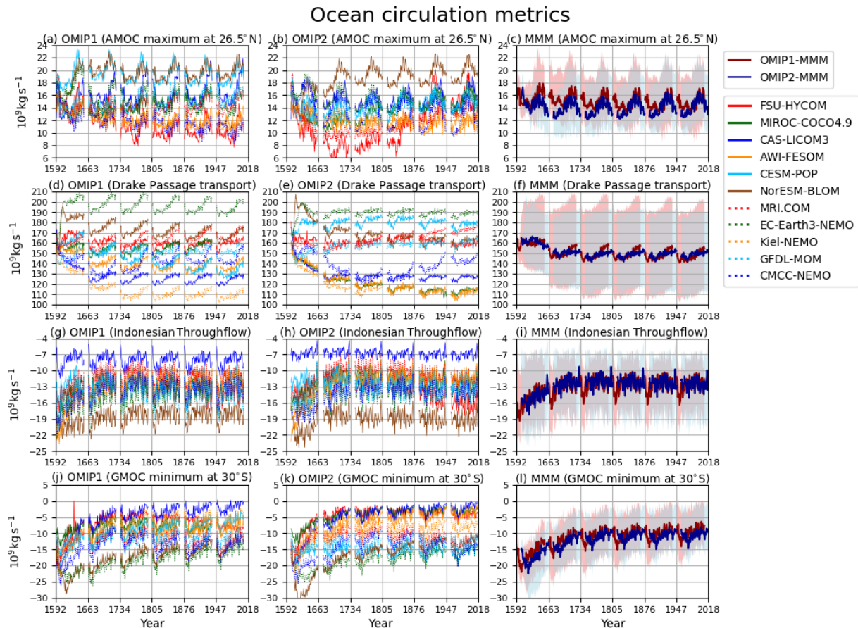
Figure 5. Time series of annual mean ocean circulation metrics. (a–c) AMOC maximum at 26.5^{\circ} N, which approximately represents the strength of AMOC associated with the North Atlantic Deep Water formation. (d–f) Drake Passage transport (positive eastward), which represents the strength of Antarctic Circumpolar Current. (g–i) Indonesian Throughflow (negative into the Indian Ocean), which represents water exchange between the Pacific and Indian oceans. (j–l) Global meridional overturning circulation (GMOC) minimum in 2000-m-bottom depths at 30^{\circ} S, which represents the strength of deep to bottom layer GMOC associated with the Antarctic Bottom Water and Lower Circumpolar Deep Water formation. (a, d, g, j) OMIP-1 and (b, e, h, k) OMIP-2. (c, f, i, l) Multi-model mean (lines) and spread defined as the range between maximum and minimum (shades) of OMIP-1 (red) and OMIP-2 (blue). Units are 10^9 \text{ kg s}^{-1} . See Figs. S8 and S9 for a closer look at individual models.
