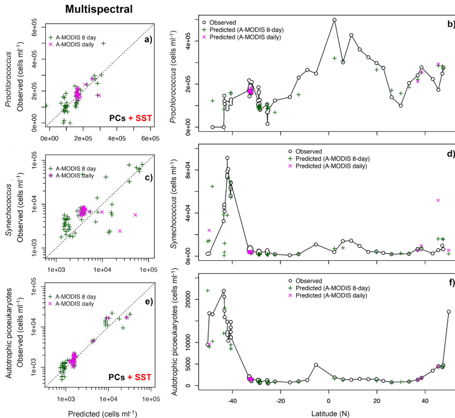
Fig. 7. Performance of developed models ( \text{PCA}_m approach) for a,b Prochlorococcus (first row), c,d Synechococcus (second row) and e,f autotrophic picoeukaryotes (third row) cell abundance, implemented using Aqua-MODIS retrievals for the cruise AMT24. In panels c and e , abundances of Synechococcus and picoeukaryotes are plotted in \log_{10} scale because this transformation was implemented for model development. SST was used as an additional predictor for models to predict Prochlorococcus and autotrophic picoeukaryotes.
