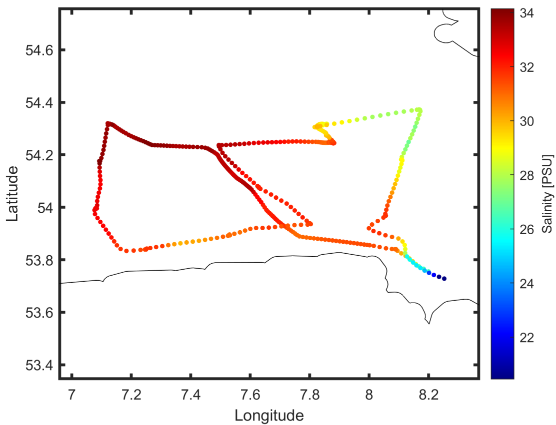
Figure 2: Cruisemap of HE549.
