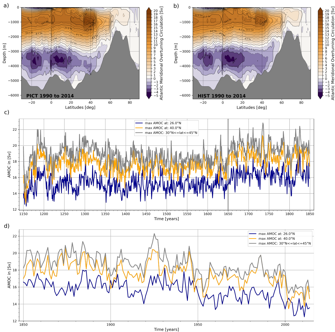
Figure 12. a) Atlantic Meridional Overtuning Circulation (AMOC) streamfunction averaged over the last 25 years in the pre-industrial control (PICT) simulation. b) as a) but for the historic (HIST) simulation. c) Evolution of the AMOC maximum at different latitudes throughout the spinup simulation (SPIN) that precedes both PICT and HIST. d) Evolution of the AMOC during HIST.
