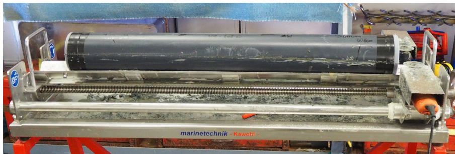
Fig. 5.2.2.9: Splitting of a core section in working and archive halves, using the Fa. Marinetechnik Kawohl vibration saw tool
