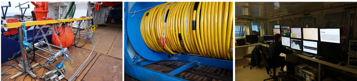
Fig. 4.1.2: Photos of GI-Gun cluster (left), winch with 600 m long digital seismic streamer (middle) and recording system monitors (right)
