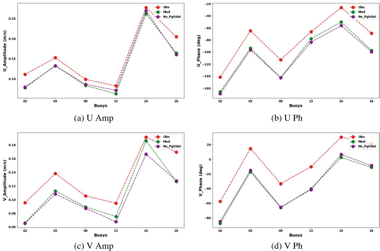
Fig. 12 Plots of M_2 amplitudes and phases of the \delta u and \delta v velocity components of the sea ice oscillations against the beacons on x - axis. The beacon observations (red colour) are compared against the point model simulations with and without pressure gradients from tidal sea surface heights. The reference point model simulation (referred to as
