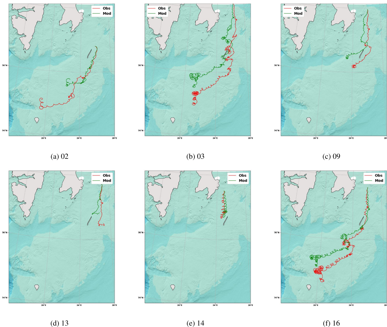
Fig. 5 Modelled drift trajectories for the beacons against the observed trajectories. The caption under each figure gives the beacon number. All the modelled trajectories are computed using a constant
