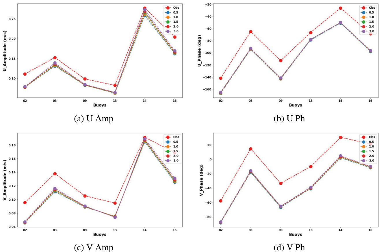
Fig. 9 Plots of M_2 amplitudes and phases ( y - axis of the \delta u and \delta v velocity components of the sea ice oscillations against the beacons on x - axis. The beacon observations (red) are compared against the
