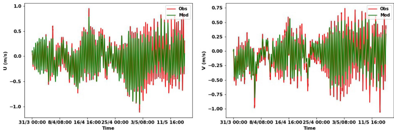
Fig. 4 Time series plot for the longitudinal ( u_i ) ( U in plot) and latitudinal ( v_i ) ( V in plot) velocities for beacon 16. Observations are in red and point model simulations are in green. Time on the x -axis is given
