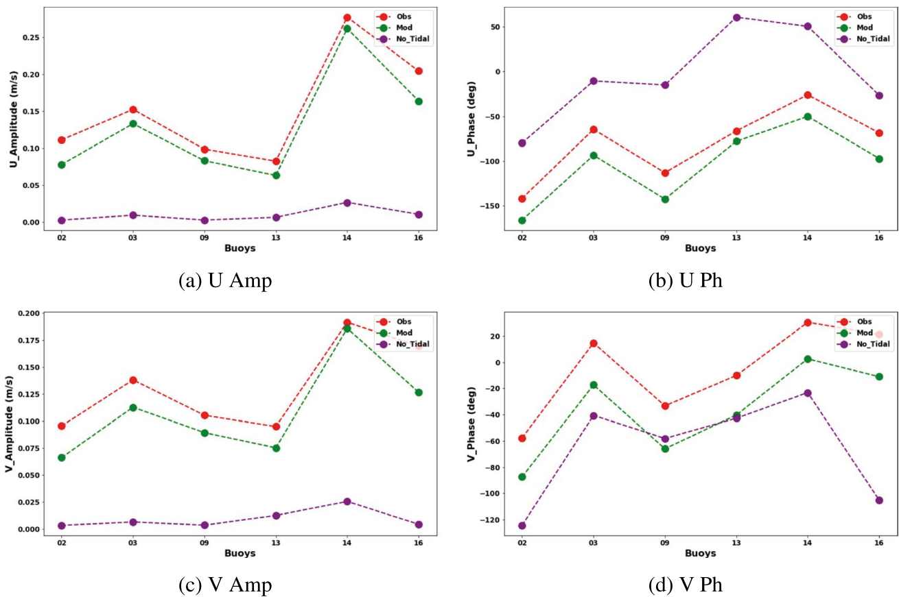
Fig. 11 Plots of M_2 amplitudes and phases of the \delta u and \delta v velocity components of the sea ice oscillations against the beacons on x - axis. The beacon observations (red colour) are compared against the point model simulations with and without tidal currents. The reference point model simulation (referred to as Mod in legend; green colour) is
