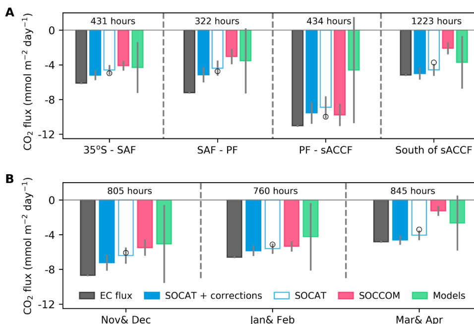
Fig. 2. Regional and temporal breakdown of the EC CO 2 flux measurements and subsampled flux estimates. In (A and B), the five bars with different colors represent the hourly EC flux measurements from the seven cruises (black), subsampled flux from SOCAT-based flux products with (filled blue) and without (unfilled blue) temperature corrections, SOCCOM-based flux products (red), and models. Open circles denote the two SOCAT-based flux products obtained using the same available interpolation methods as those for the SOCCOM-weighted products. Error bars reflecting one SD provide a measure of uncertainty (see Materials and Methods). Refer to the caption of Fig. 1 for the definition of the fronts SAF, PF, and sACCF. The number of hours of matched EC flux and subsampled flux is indicated above each subplot.
