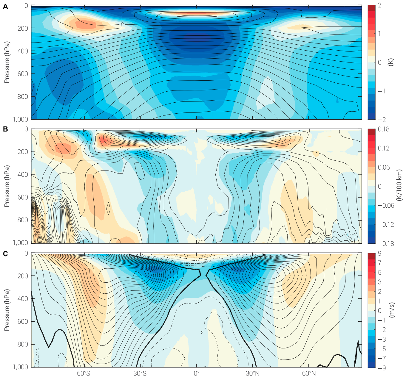
Fig. 8. Zonal-mean anomalies of (A) air temperature, (B) MTG, and (C) u-wind in the ECHAM6 sensitivity experiment with respect to the control experiment. The corresponding climatological distributions of air-temperature, MTG, and u-wind are given by the contours. For the u-wind panel, i.e., subpanel (C), positive values represent westerly wind anomalies, and vice versa. The black contours give the climatological u-wind distribution. Solid contours show westerly wind, and dashed contours are easterly wind. The thick black lines illustrate the zero-crossing of u-wind from easterly to westerly.
