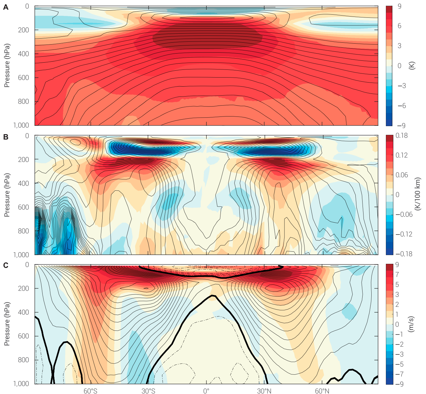
Fig. 5. Zonal-mean anomalies of (A) air temperature, (B) MTG, and (C) u-wind in the amip4K experiment with respect to the amip control experiment. The corresponding climatological distributions of air temperature, MTG, and u-wind are given by the contours. For the u-wind panel, positive values represent westerly wind anomalies, and vice versa. The black contours give the climatological u-wind distribution. Solid contours show westerly winds, and dashed contours are easterly winds. The thick black lines illustrate the zero-crossing of u-wind from easterly to westerly. The poleward shift of the tropospheric jet stream is visible in the amip4K experiment with westerly/easterly wind anomalies at the poleward/equator flanks of climatological position of westerly jets. The results are based on the ensemble mean of 7 model outputs from the CMIP5.
