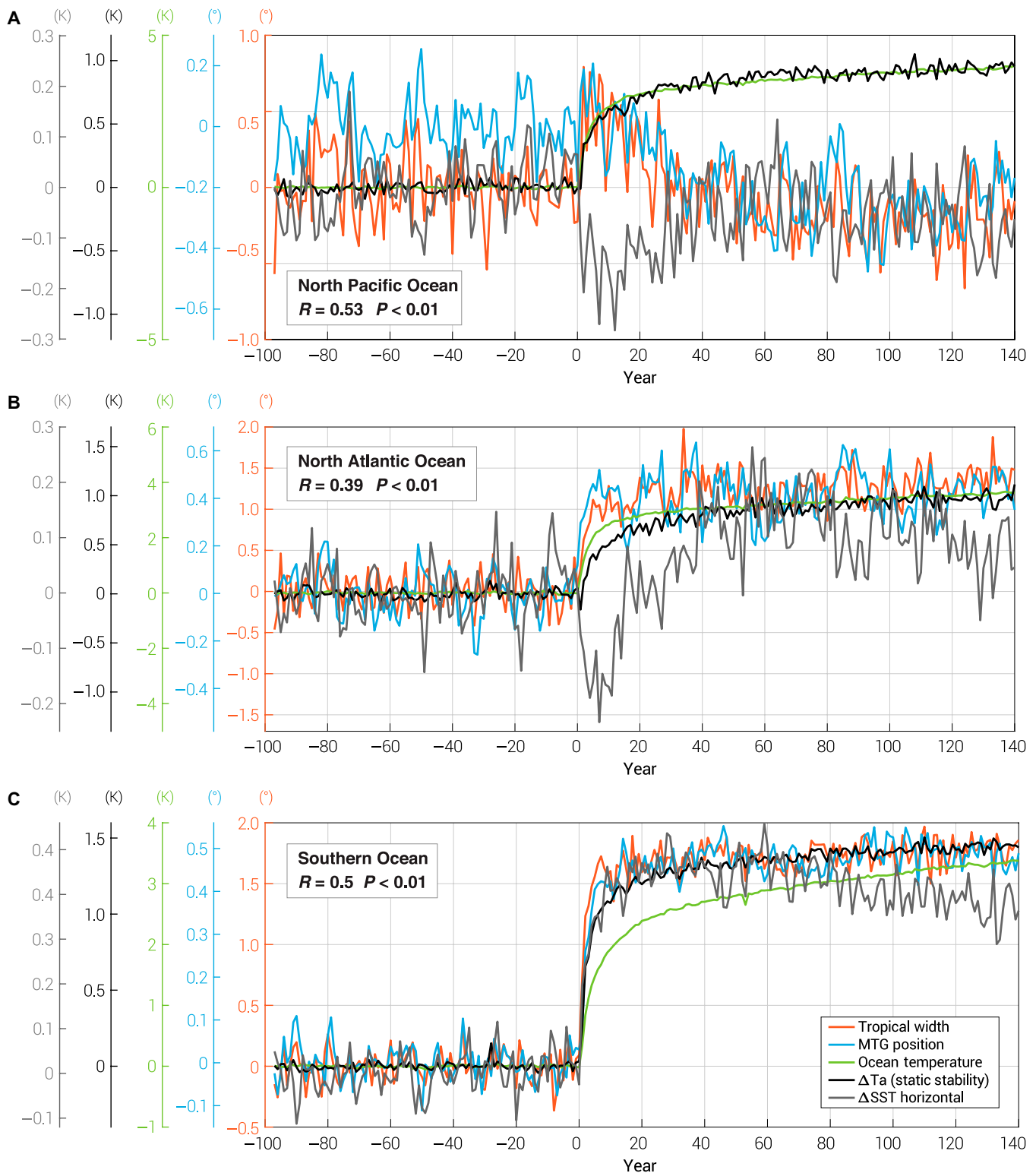
Fig. 3. Anomalies of tropical width (red lines), meridional migration of MTG (blue lines), ocean surface temperature (green lines), subtropical static stability (black lines), and horizontal SST gradient (gray lines) in the last 100 years of the piControl experiment (left) and 140 years of abrupt4xCO 2 experiments (right). (A) For North Pacific Ocean. (B) For North Atlantic Ocean. (C) For Southern Ocean. Detailed definitions of these variables can be found in Materials and Methods. The ensemble-mean correlation coefficients between the tropical width and MTG position in the abrupt4xCO 2 experiment are given by R , with corresponding P values provided by P (Student's t test). All time series are shown as anomalies with respect to the corresponding piControl experiment.
