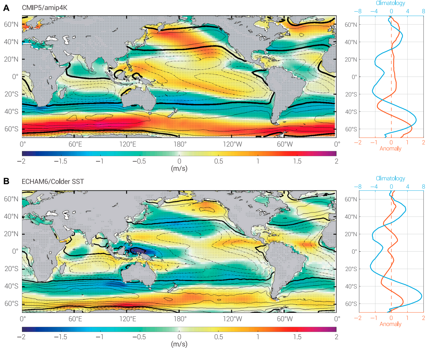
Fig. 6. Poleward shift of near-surface zonal wind in (A) CMIP5 ami4K and (B) ECHAM6 global cooling experiments. The shading illustrates the near-surface wind anomalies in the sensitivity experiments (i.e., ami4K and ECHAM6 cooling experiment) with respect to the corresponding control experiments (i.e., ami and ECHAM6 control experiment). The contours illustrate the climatology near-surface zonal wind. Dashed lines represent easterly winds, while solid lines illustrate westerly winds. The thick black lines are the zero-crossing of zonal wind. The right panels depict the zonal mean profile of the climatology (blue) and anomaly (red) of zonal winds. For the CMIP5 result, stippling indicates that more than 5 of 7 models agree on the signs of the anomalies. For the ECHAM6 result, stippling represents that the anomalies are statistically significant (pass the 95% confidence level, Student's t test).
