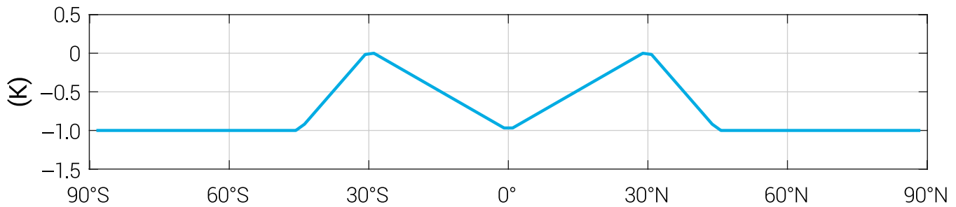
Fig. 2. Zonal-mean anomalies of SST in the ECHAM6 sensitivity experiment with respect to the control experiment.
