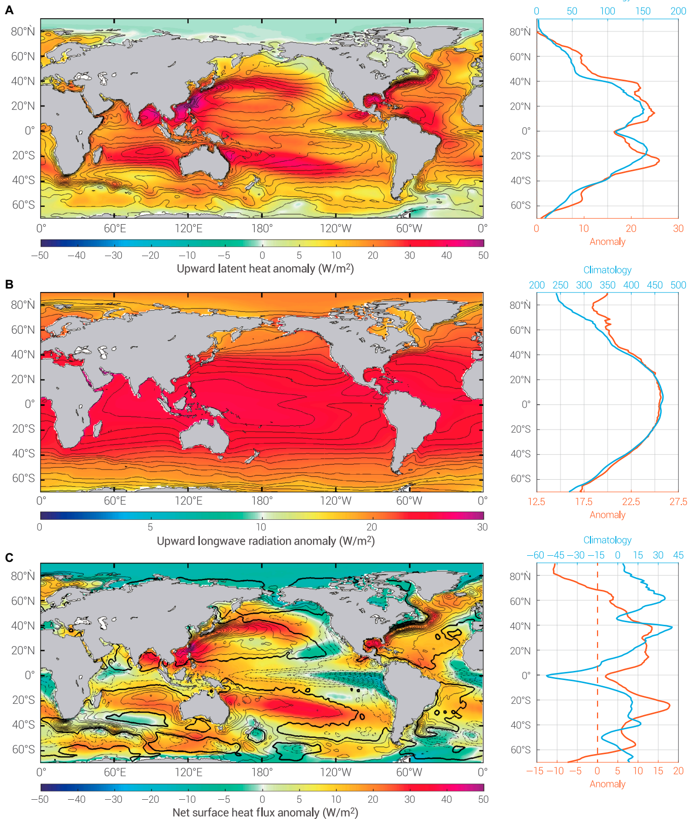
Fig. 7. Anomalies of (A) latent heat flux, (B) upward thermal radiation, and (C) net surface heat flux in the amip4K experiment with respect to the amip control experiment. The contours illustrate the climatology distribution of different heat fluxes. For the net surface heat flux, solid lines represent oceanic heat release into the atmosphere, and dashed lines indicate net ocean heat gain. The contour interval is 15 \text{ W/m}^2 . The results are based on the ensemble mean of 7 CMIP5 model outputs.
