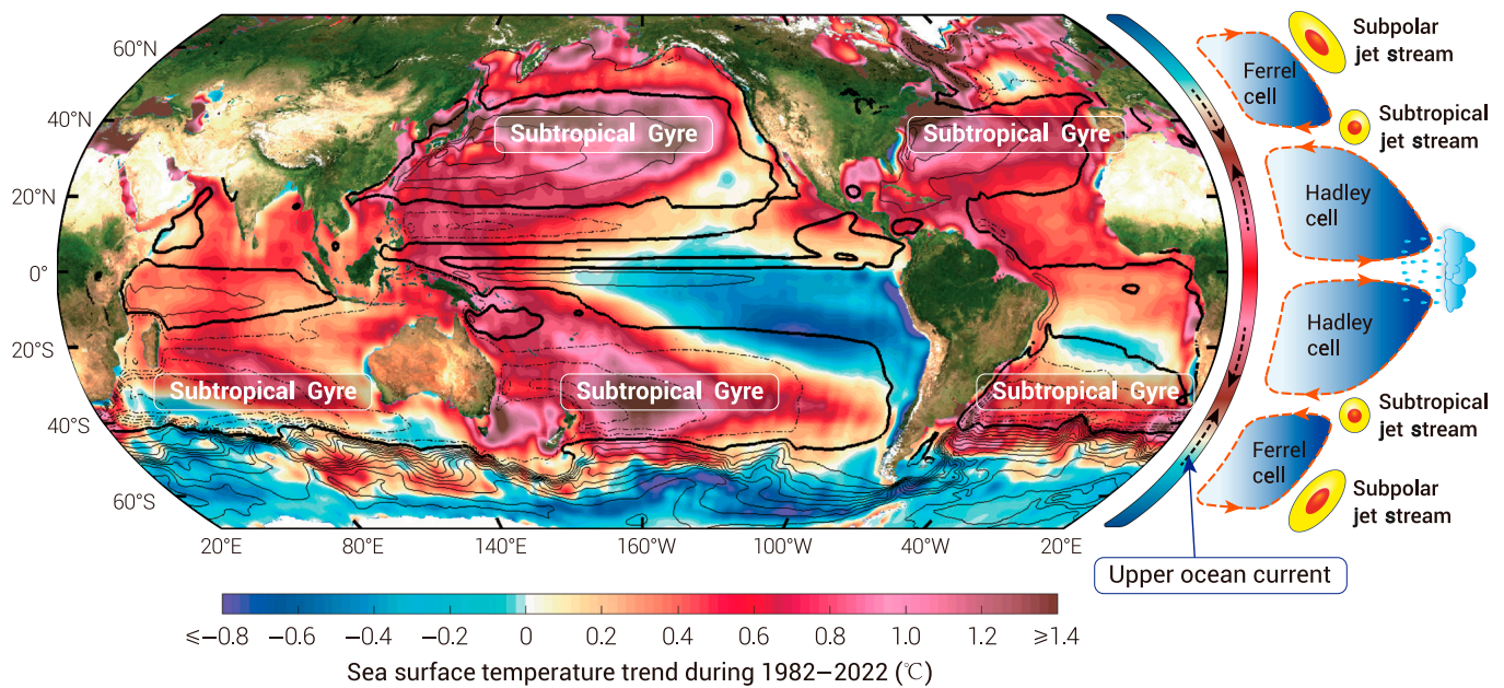
Fig. 1. Schematic diagram showing how the background subtropical gyres promote enhanced subtropical ocean warming and drives tropical expansion. Shading indicates the SST trend during the satellite era (1982 to 2022). Contours present the climatological oceanic barotropic stream function [69], which locates the major subtropical ocean gyres. On the right panel, the arrows illustrate the significant features of atmospheric (red) and upper oceanic (black) circulation. Under the forcing of increasing greenhouse gases, background subtropical ocean gyres promote enhanced subtropical ocean warming by converging the upper ocean water. The enhanced subtropical warming expands the low latitude warm water zones, pushes the mid-latitude MTGs toward higher latitudes, and thus forces tropical expansion. Figure modified from Yang et al. [10]. The National Oceanic and Atmospheric Administration OISSTv2 data [70] were used to calculate the linear SST trend.
