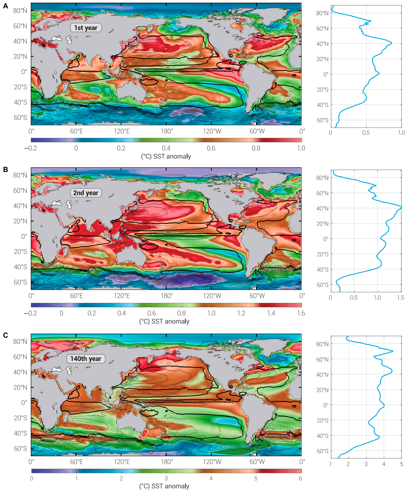
Fig. 4. The SST anomalies in the (A) very 1st year, (B) 2nd year and (C) 140th year of the abrupt4xCO 2 experiment. The SST anomalies for individual years are given with respect to the climatology SST of the piControl experiment. To illustrate the region where surface water converges (subtropical ocean gyres), the climatology barotropic stream function of oceanic circulation [69] is overlapped by the black contours. The right panels present the zonal mean SST anomaly. At the onset of the abrupt4xCO 2 experiment, the subtropical ocean gyres exhibit a relatively strong surface warming. This relatively strong subtropical ocean warming causes a rapid poleward shift of the mid-latitude MTG, as shown in Fig. 3 (blue lines). Over the North Pacific Ocean, the long-term warming pattern induces a relatively weak subtropical warming and an equatorward shift of the mid-latitude MTG, contributing to a long-term regional contraction of the tropical belt as shown in Fig. 3A (red line). The results are based on the ensemble mean of 17 CMIP5 model outputs.
