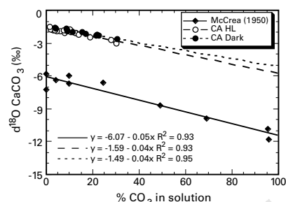
Figure 4 Comparison of high light and dark O. universa \delta^{18}\text{O} data from the constant alkalinity (CA) experiment with inorganic precipitate results from McCrea 18 . Oxygen isotope data are plotted against % \text{CO}_3^{2-} in solution, where \% \text{CO}_3^{2-} = \frac{[\text{CO}_3^{2-}]}{([\text{CO}_3^{2-}] + [\text{HCO}_3^-])} \times 100 . Note that the slopes of our experimental data are indistinguishable from that obtained by McCrea.
