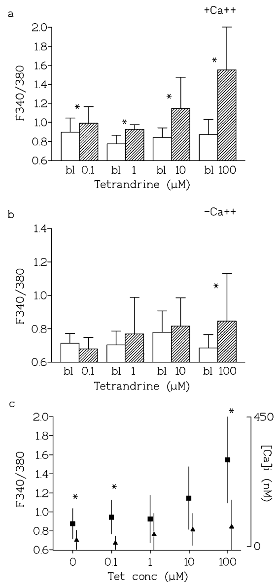
Fig. 5 a Elevation of fluorescence ratio induced by various concentrations of tetrandrine in calcium-containing buffer. bl represents baselines in cells before treatment. * P < 0.05 , Anova for repeated measures, Wilcoxon signed rank test. Each column represents data from at least 14 cells. b Elevation of fluorescence ratio induced by various concentrations of tetrandrine in calcium-free buffer (2–3 min). bl represents the baseline of cells before treatment. * P < 0.05 , Anova for repeated measures, Wilcoxon signed rank test. Each column represents data from at least 9 cells. c Elevation of [Ca]_i induced by various concentrations of tetrandrine in the presence (■) and in the absence of extracellular calcium (▲). Each point represents the result from at least 9 cells. * P < 0.05 between both conditions at the same concentration
