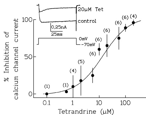
Fig. 1 Inhibition of calcium channel currents of chromaffin cells by various concentrations of tetrandrine, measured in the whole cell configuration of the patch clamp technique. The number of cells treated with equal concentrations is indicated above the error bars. The IC_{50} was 10.4 \mu\text{M} . Cells were clamped to -70 \text{ mV} and depolarized to 0 \text{ mV} for 100 \text{ ms} as indicated in the inset which shows a current trace during treatment with 20 \mu\text{M} tetrandrine
